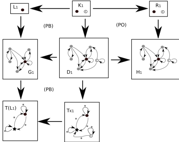
Figure 4: Rule for copying a web page and example of application.
