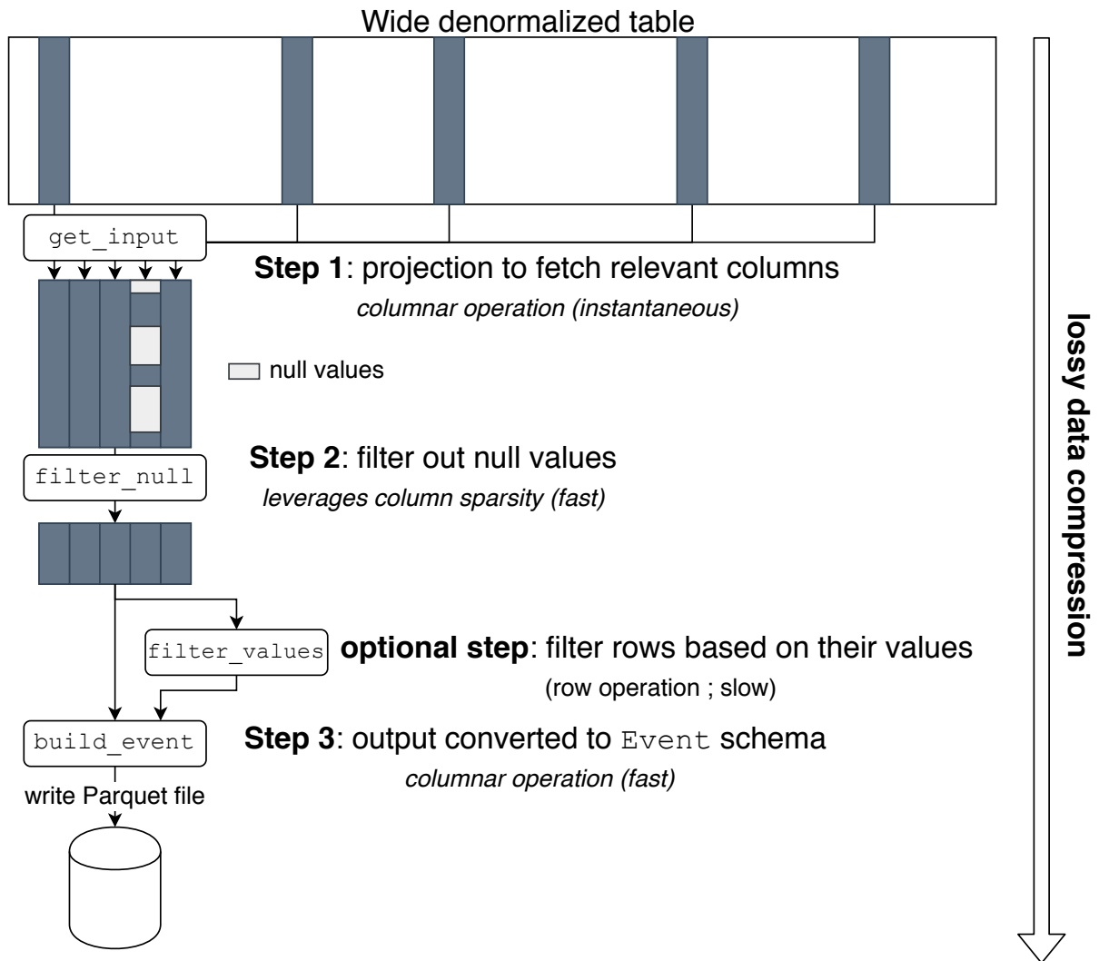
Figure 2: Extractor design. Extractors implemented in SCALPEL-Extraction successively refines the input table (a large denormalized table) by taking advantage of fast columnar operations to produce ready-to-use medical events. Step 1 selects the relevant columns (equivalent to a hash table look-up) while Step 2 removes rows where null values are detected in specific columns, taking advantage of the sparsity of columnar representation (null values are not encoded in the data). Optionally, this extraction process filters out rows based on their values. Finally, Step 3 conforms the data to the Event schema, and is written to a Parquet file.
