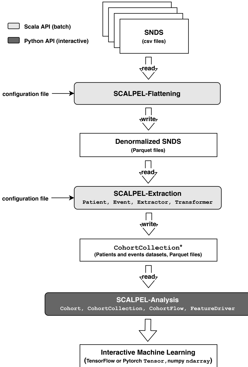
Figure 1: SCALPEL3 workflow. SCALPEL3 is made of three independent open-source libraries plugged one after another. SCALPEL-Flattening, which is implemented in Scala/Spark, denormalizes the input database exported as CSV or Parquet files into a single big flat database. Then, SCALPEL-Extraction, implemented in Scala/Spark, extracts concepts from this flat database. Finally, SCALPEL-Analysis, implemented in Python/PySpark loads extracted concepts to perform in-memory interactive analysis and feed machine learning algorithms.
