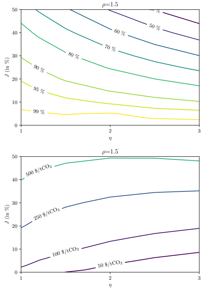
Figure 5: CRRA preferences. Sensitivity analysis for T_{max} = 10^{\circ}C . Top panel: Contour of share of SCC explained by expected damages (ratio of SCC deterministic on SCC stochastic). Bottom panel: SCC for stochastic runs (in US $2005).
