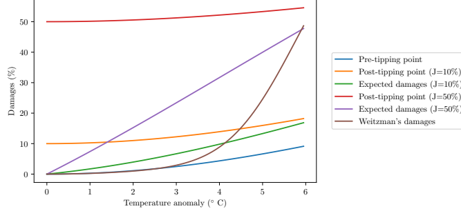
Figure 1: Comparison between different damage functions.
