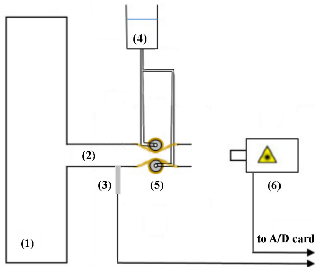
Figure 1: (Color online) Schematic of the experimental setup composed of (1) the pressure reservoir, (2) the tube supplying air to (5) the vocal folds replica, (3) the air pressure sensor, (4) the water tank, and (6) the laser vibrometer.
