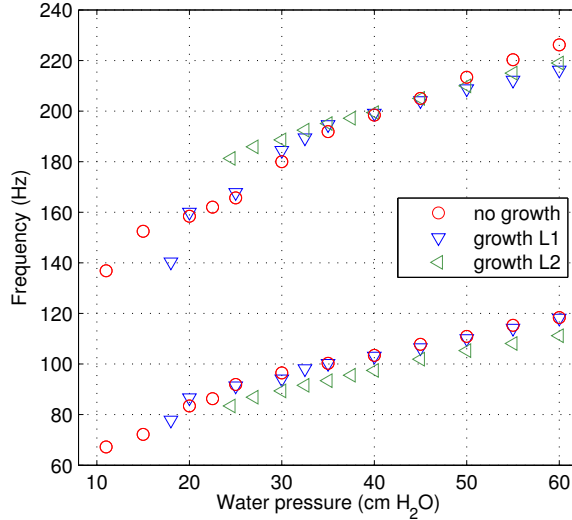
Figure 4: (Color online) Center frequency of the first two resonances against P_w , obtained from mechanical measurements (FRF), with and without growth. The estimated measurement error is 0.3 Hz, i.e. less than the size of the markers.
