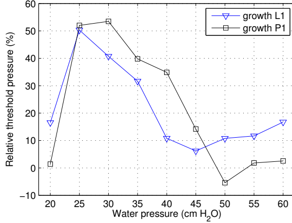
Figure 7: (Color online) Oscillation threshold pressure with the lead (L1) and plasticine (P1) growths, relative to their respective reference series without growth (Fig. 6). The series with growth L1 is the same as in Fig. 5 in the high frequency regime.
