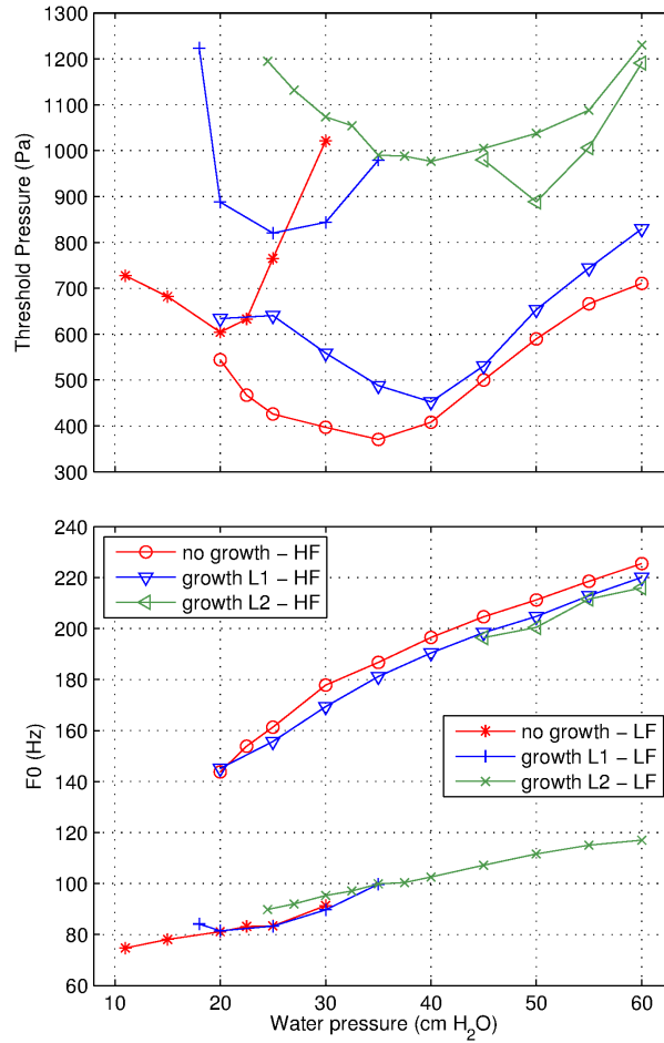
Figure 5: (Color online) Top: oscillation threshold pressure from measurements for healthy and pathological configurations in both low frequency (LF) and high frequency (HF) oscillation regimes. Bottom: Fundamental frequency of oscillation in the same conditions.
