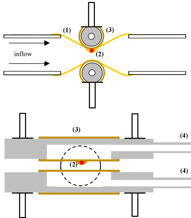
Figure 2: (Color online) Schematic of the vocal folds replica in side view (top) and front view (bottom). (1) Latex tube connection, (2) growth made of a small solid ball stuck between the latex membranes 1 and 3, (3) latex tubes filled with water, (4) connections to the water tank.
