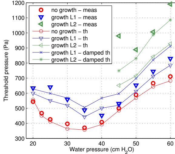
Figure 10: (Color online) Oscillation threshold pressure in high frequency regime from the theoretical model of oscillation without (“th”) and with (“damped th”) initial contact, i.e. damping according to Eqs. (4) & (5) respectively, between the vocal folds, compared to measurements from the vocal fold replica.
