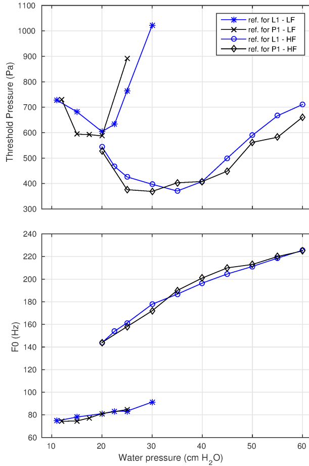
Figure 6: (Color online) Reference series (without growth) of oscillation threshold pressure (top) and fundamental frequency F0 (bottom) for the lead (L1) and plasticine (P1) growths. The reference series for growth L1 is the series without growth presented in Fig. 5.
