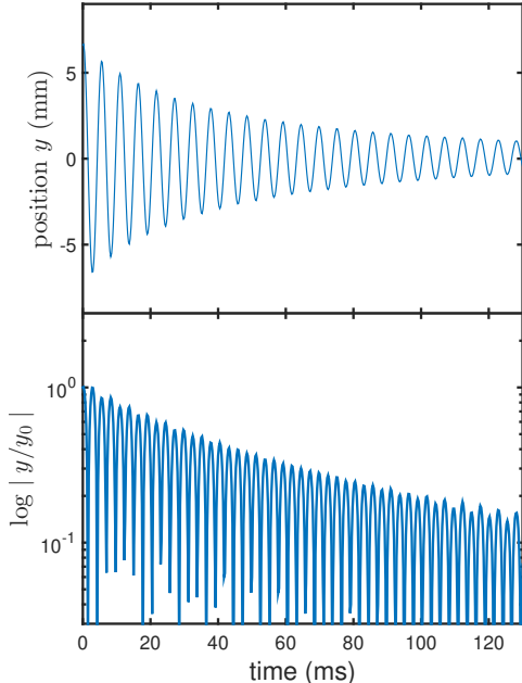
FIG. 3. Free oscillations of the free end of a clamped wooden stick (Wood 2 in table I) in linear (top) and log (bottom) scales. Measuring the frequency leads to the value of the Young’s modulus of the stick. The damping is caused by internal dissipation within the stick.
