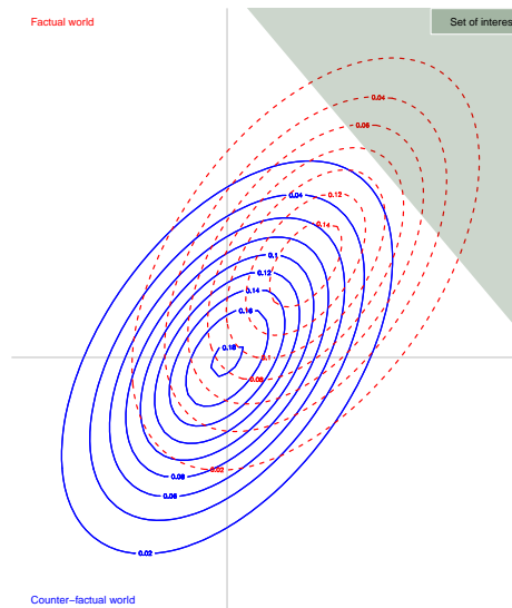
FIGURE 1 Classical scheme used in EEA: A counterfactual world (solid contours of the bivariate pdf) represents a world without any anthropogenic influence and a factual world (dotted contours of the bivariate pdf) corresponds to our actual climate. For example, the x-axis and y-axis could represent mean decadal summer temperatures at two different locations. The main EEA question is to compare the probability of being in the set of interest (greenish area) with respect to the two worlds. In this figure, the event of interest could be the average temperature between the two locations being large.
