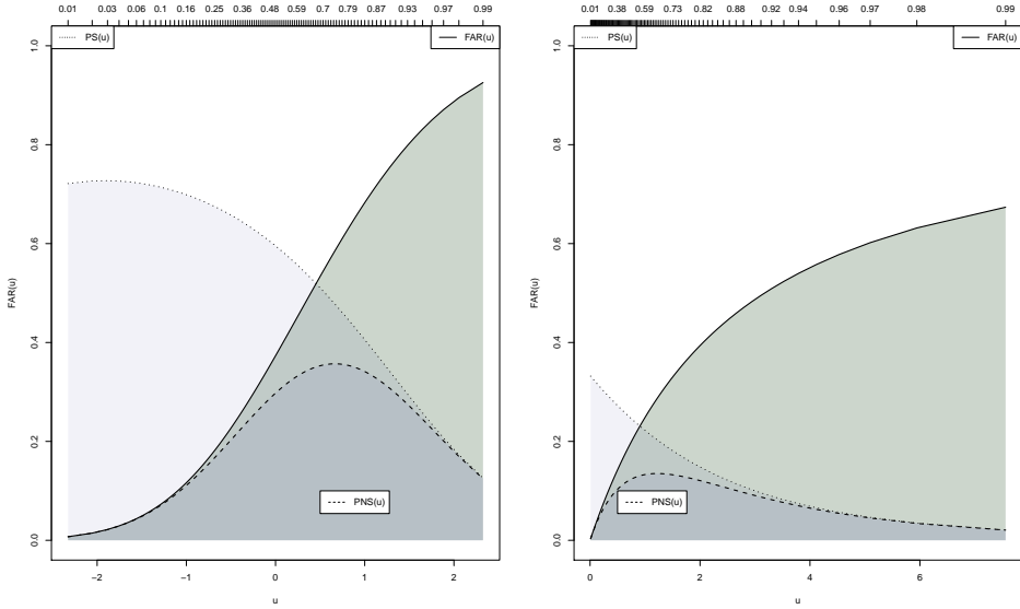
FIGURE 2 FAR(u) (solid line), probability of sufficient causation (dotted lines) and probability of sufficient and necessary causation (dashed lines) in function of the threshold u , see Equation (2). The left and right panels correspond to the Gaussian and Pareto cases, respectively.
