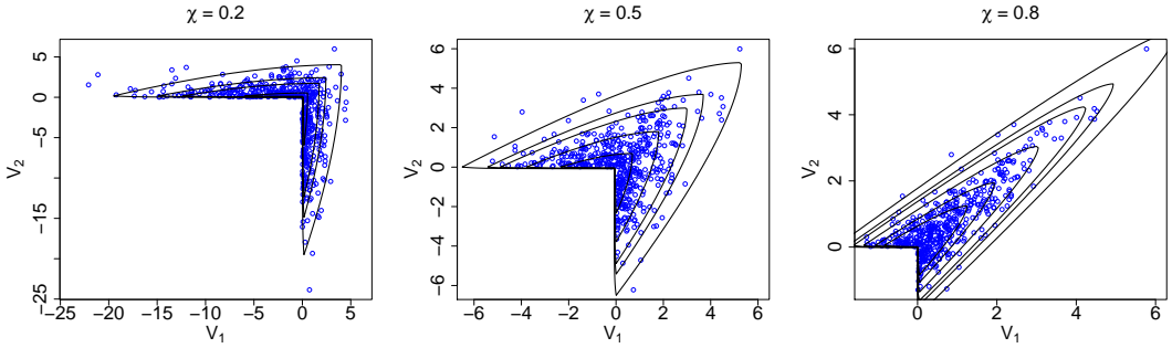
FIGURE 3 Scatterplots and density contours for the bivariate Gaussian MGPD model (12) with \xi = (0, 0) , \sigma = (1, 1) , \beta = (0, 0) . From left to right, the tail dependence coefficient (13) equals to \chi = 0.2 , \chi = 0.5 and \chi = 0.8 .
