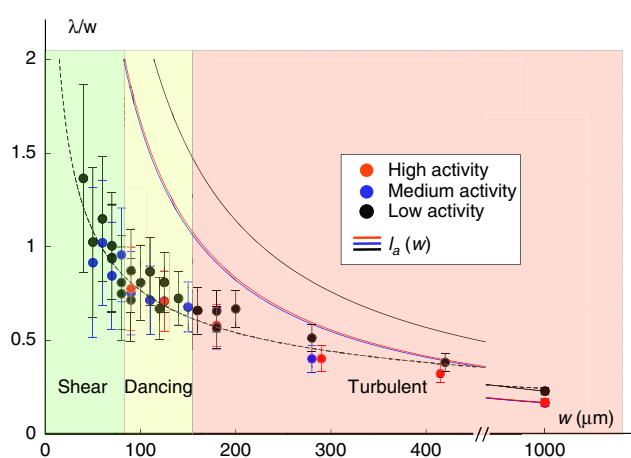
Fig. 2 Defect Spacing. Experimental mean defect spacing, \lambda , rescaled by the channel width, w , as a function of w . Different colours correspond to different activities. The error bars correspond to the standard deviation for measurements at 10 random times for each experiment. The non-scaled data is displayed in Supplementary Fig. 2. The dotted line corresponds to a fit with w^{-1/2} . The continuous lines correspond to \lambda/w = l_a/w for each experiment, with l_a being the active length scale corresponding to the value of \lambda in the unconfined case
