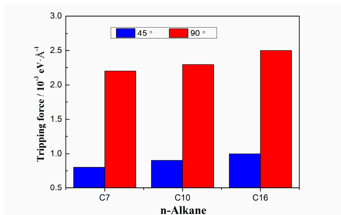
Figure 3. Tripping forces of water/ n -alkane/solid systems.
