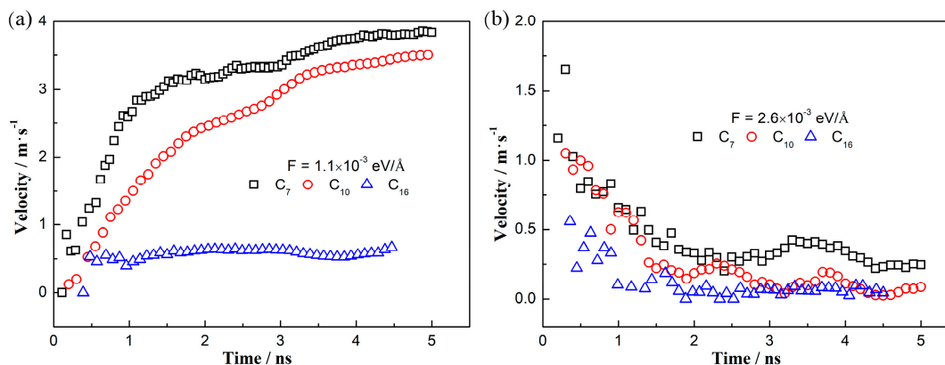
Figure 4. Contact line velocity versus time for the water/ n -alkane/solid systems with different molecular chain length. (a) Wettability of 45°. (b) Wettability of 90°.
