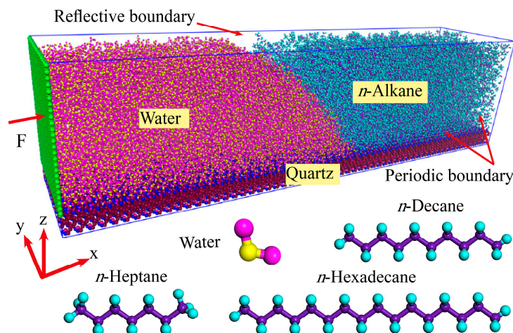
Figure 1. Simulation model of the displacing process in the water/ n -alkane/quartz systems. Structures of water and n -alkanes, heptane (C 7 ), decane (C 10 ), and hexadecane (C 16 ) are given.
