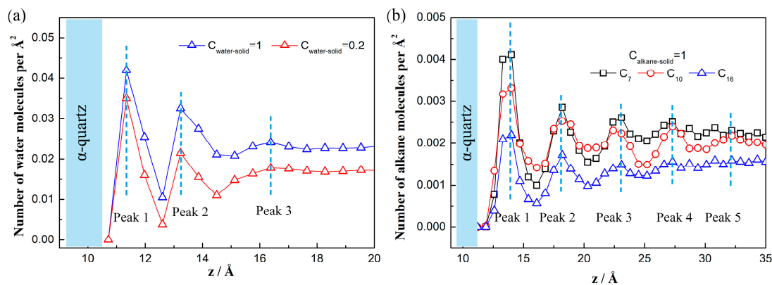
Figure 2. Number density near a quartz surface along the z -coordinates. (a) Water molecules. C is the liquid-solid energy coefficient. Blue lines represent a contact angle of 45^\circ and red lines a contact angle of 90^\circ . (b) n -Alkane molecules.
