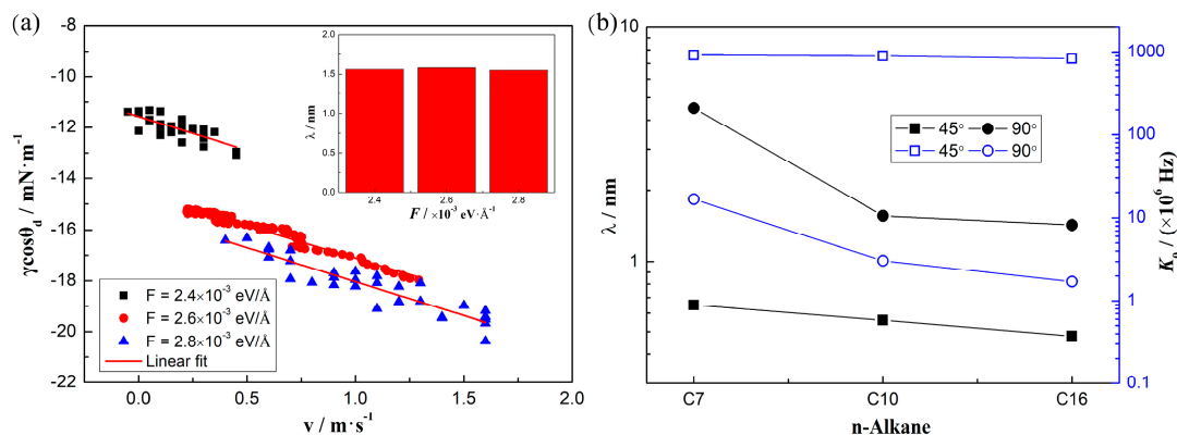
Figure 5. Jump mean distance \lambda and frequency K_0 of the molecular displacement occurring within contact line zone, obtained by the molecular-kinetics theory. (a) The case of water/n-decane/solid system with the wettability of 90^\circ : linear fitting of the molecular-kinetics theory and the jump mean distance under different driving forces. (b) The black one represents the mean distance and the blue one represents the frequency.
