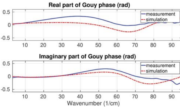
Fig. 2 Comparison of the measurement (blue curve) and simulation (red dashed curve) of the complex Gouy phase corresponding to the measurement of the high resistivity silicon.
