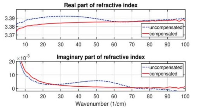
Fig. 1 Real and imaginary part of complex refractive index of high resistivity silicon are shown. Uncompensated (dashed blue line) and compensated (full red line) complex refractive indices differ in the Gouy phase influence [3].
