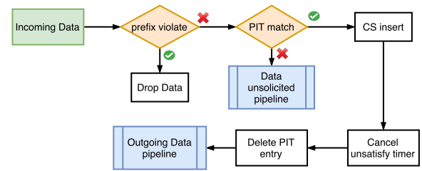
Figure 3: Incoming Data pipeline
