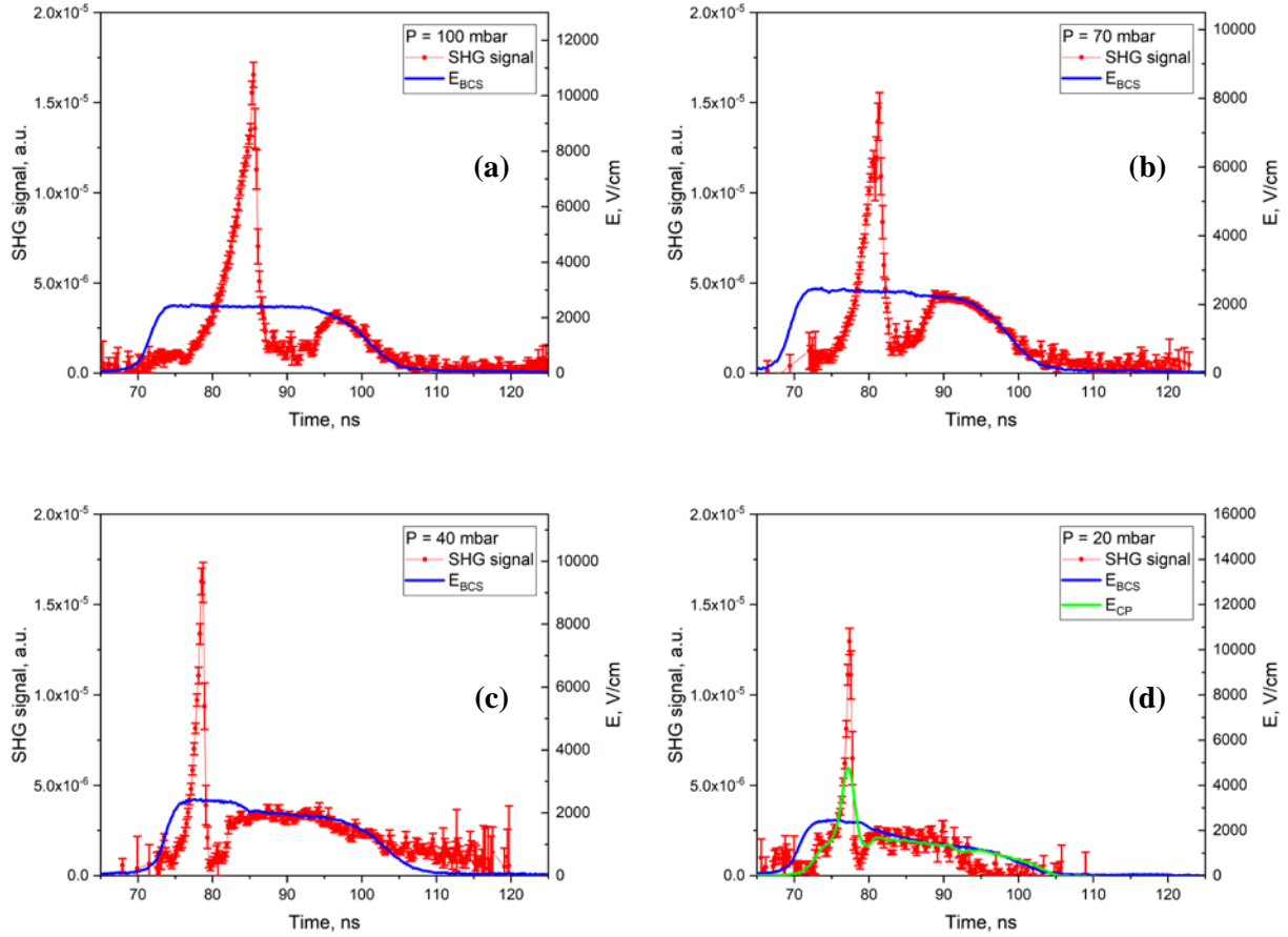
Figure 6. Electric field in a fast ionization wave discharge in nitrogen at P=20 -100 mbar, plotted together with the current shunt signal used for absolute calibration (EBCS). Electric field inferred from the capacitive probe measurements (ECP) is also plotted at P=20 mbar.
