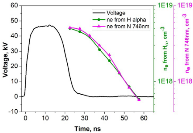
Fig. 5. Electron density measured from H \alpha and nitrogen (746 nm) corresponding with voltage.
