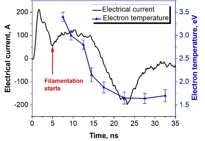
Fig. 3. Measured electron temperature corresponding synchronized with electrical current.
