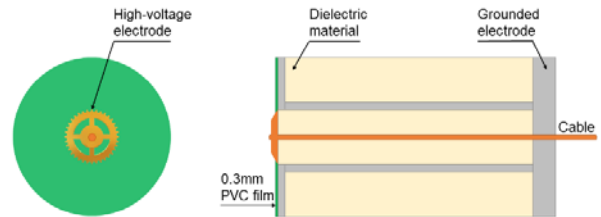
Fig. 1. Configuration of cylindrical electrode system.
