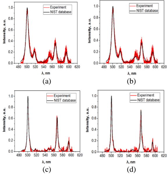
Fig. 2. Experimental (red curves) and calculated (black curves) spectra (a)(b) in discharge; (c)(d) in afterglow.
