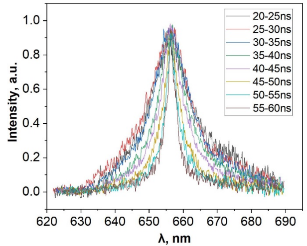
Fig. 4. H_\alpha line Stark broadenings at different time steps.
