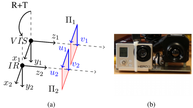
Fig. 1. (a) The layout of our stereo acquisition system. VIS and IR are respectively the visible and the infrared camera, \Pi_1 and \Pi_2 are the image planes of respectively camera VIS and IR. R : rotation matrix from camera VIS to camera IR, T : translation matrix from camera VIS to camera IR. (b) Picture of our stereoscopic system.
