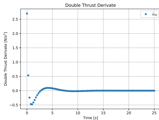
Figure 9: PVTOL Double Thrust Derivate
