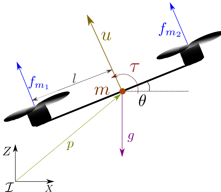
Figure 1: The PVTOL free body diagram.
