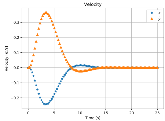
Figure 3: PVTOL Velocity
