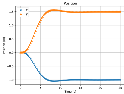
Figure 2: PVTOL Position
