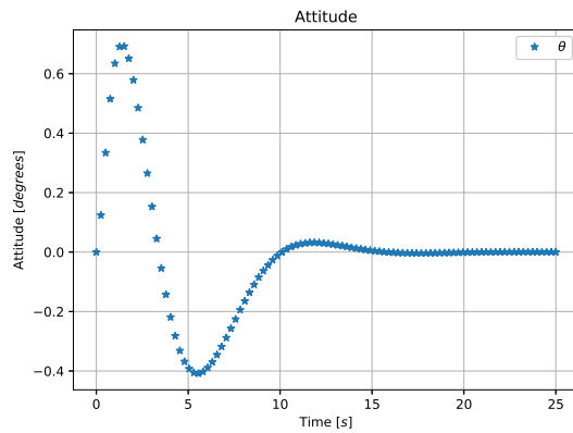
Figure 4: PVTOL Attitude
