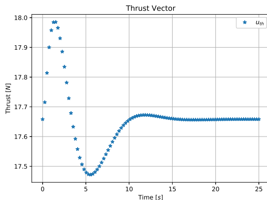
Figure 7: PVTOL Thrust Vector
