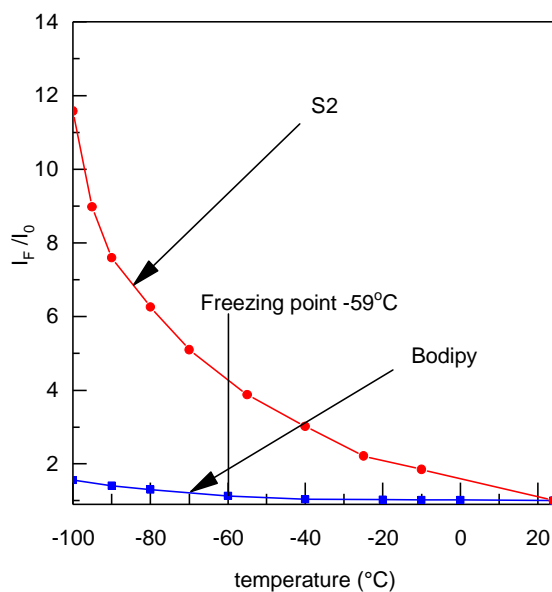
Figure 5. Comparison of fluorescence spectra changes of reference BODIPY (Blue) and S2 (red) in propylene glycol at different temperatures. [S2] = 10 \mu M, \lambda_{exc} = 365 nm, \lambda_{obs} = 520 nm. [BODIPY] = 10 \mu M, \lambda_{exc} = 510 nm, \lambda_{obs} = 530 nm.
