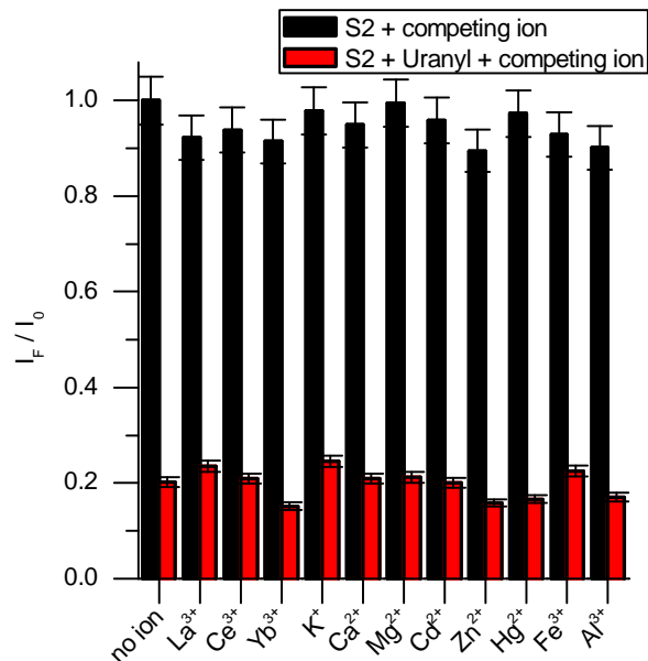
Figure 8. Selectivity of S2 towards uranyl over other metal ions. Reaction time is one hour. Excitation wavelength was 365 nm and all fluorescence values were recorded at 550nm. [S2] = 7 \mu M, [UO 2 2+ ] = [competing cations] = 20 \mu M. Uranyl source: uranyl nitrate.
