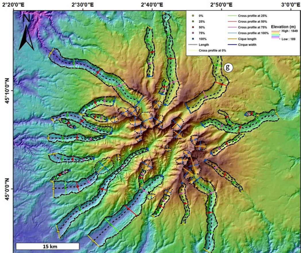
Figure 9: Study area in Cantal in French Massif Central on Earth. Colorized elevation data from 25m/pixel DEM. The white circle is the valley represented in the Fig.11 Images credit IGN.
