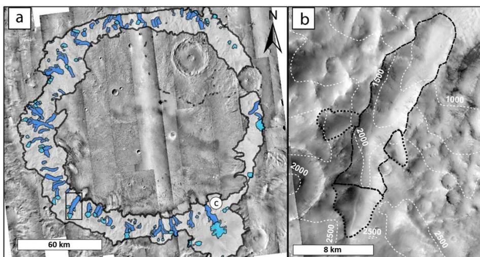
Figure 8: Dawes crater (a) Background using CTX images. The dark and light blue represents respectively the glacial valleys and the glacial cirques. (b) CTX detailed view of the glacial valleys surrounding by three glacial cirques shown in (a). Modified from (Bouquety et al., 2019). The white circle is the valley represented in the Fig.11. Images credit NASA/JPL/University of Arizona.
