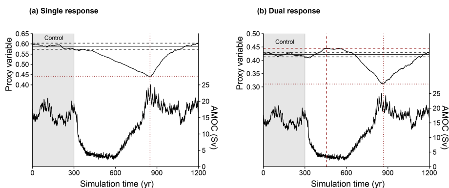
Figure 2. Theoretical definition of the proxy response studied (dotted red horizontal line) and the time of response (dotted vertical red line) in the case of (a) a single response or (b) a dual response to the circulation change induced by the freshwater addition. In the case of dual response, we examine the early (i.e. the first) and the late (i.e. the second) proxy response and time of response. The anomaly is defined as the difference between the proxy value at the defined time of response and the average proxy value (horizontal black line) during the control period of 300 years (highlighted in grey). The horizontal dashed black lines represent the proxy variance ( 2\sigma ) over the control period (highlighted in grey). The proxy variable used is purposely not specified since the interest here is to provide an illustration of the definition used in the present study with the different modelled proxy variables.
