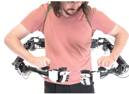
Figure 1: The Co-Limbs user interface uses force sensors and admittance control to enable a user to intuitively move and use the otherwise non-backdrivable wearable robotic arms.
