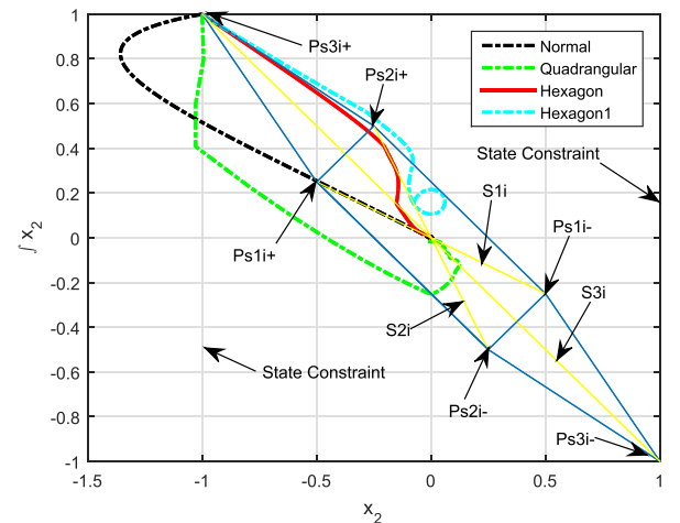
FIGURE 8. Point (x_2, \int x_2) trajectory.
