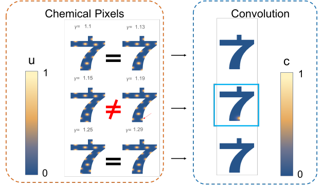
Fig. 5 FEM simulations of steady states for pairs of Turing nodes with close chemical strength \gamma (plotting u in each Turing node) and the corresponding convolution layer. Color bars are in arbitrary units of density
