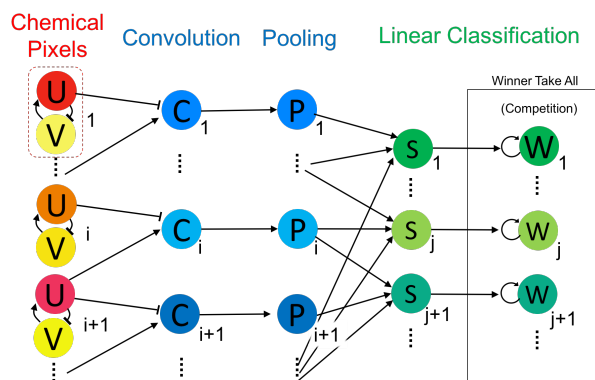
Fig. 1 Illustration of the general architecture of the swarm. The first layer contains "chemical pixels", which are pairs of agents forming a Turing pattern. The convolution layer acts as an "edge detector", picking up differences between chemical pixels. Lastly the pooling layer averages concentration at the scale of the reactor, and the last layer classifies the resulting signatures to recognize the shape of the reactor.
