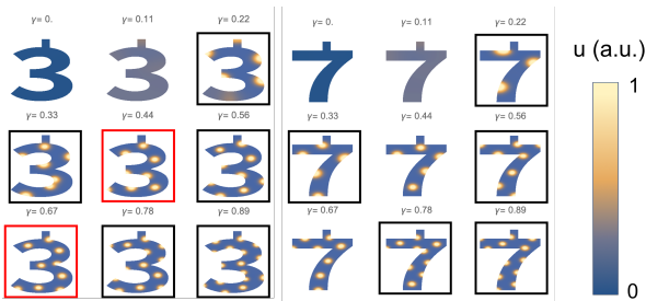
Fig. 4 FEM simulations of the Turing for two geometries and various chemical strength \gamma patterns. Color bars are in arbitrary units of density
