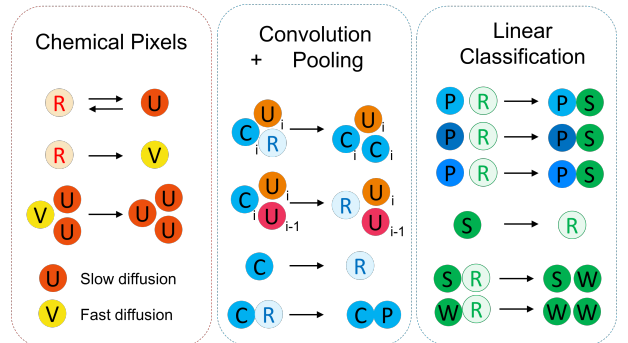
Fig. 3 Chemical reactivity rules. In this paper, we implement the chemical pixels and the convolution layer.
