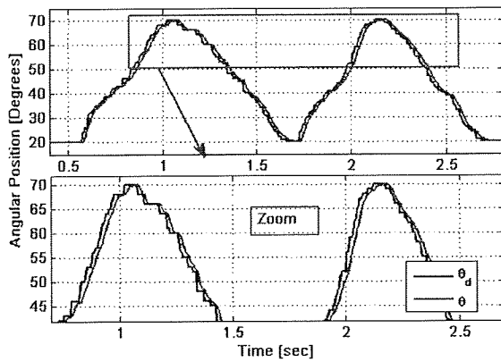
Fig. 6. Real-time experimental results of trajectory tracking generated by a signal obtained by a force sensor when flexes and extends the elbow joint.
