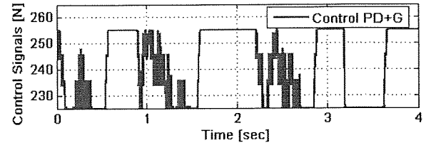
Fig. 9. Real-time control signal of the PD + G control applied to all actuators for the trajectory-tracking test.
