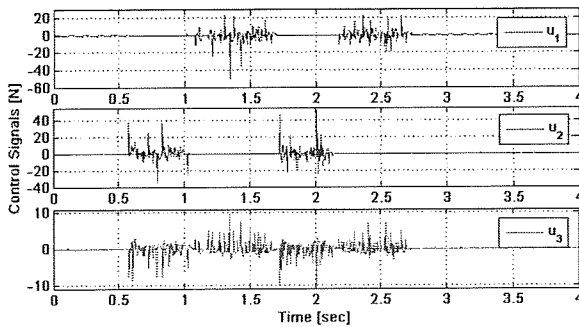
Fig. 7. Real-time control signals ( u_1 , u_2 , and u_3 ) corresponding to the pneumatic muscles and electric motor for the trajectory-tracking test.
