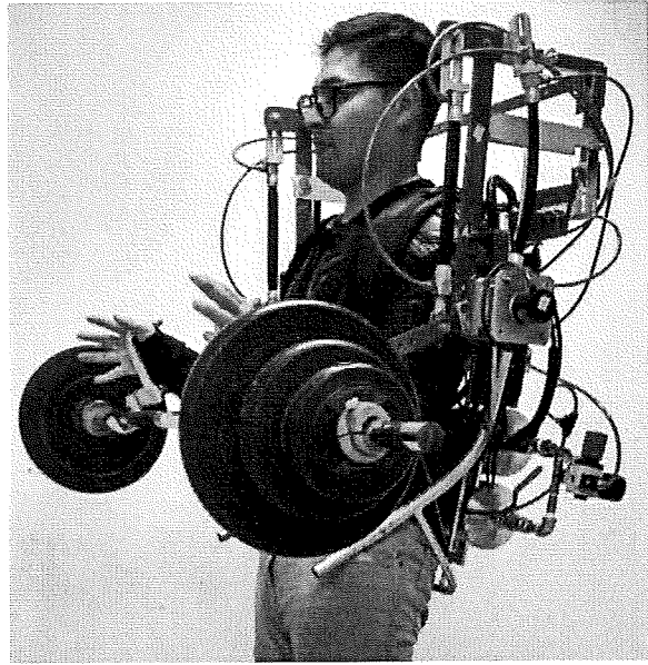
Fig. 1. Force augmenting hybrid exoskeleton for the elbow joints.
