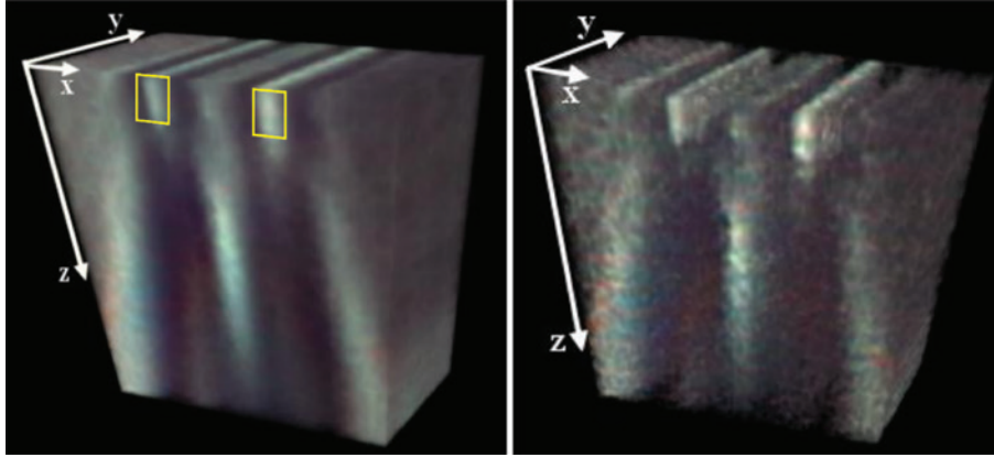
Figure 6: White-light 3D intensity distributions diffracted by a pair of parallel polymer lines separated by 2\ \mu\text{m} . Left: raw z-stack images. Right: deconvoluted z-stack images. Yellow rectangles represent line profiles ( W=0.4\ \mu\text{m} and H=0.9\ \mu\text{m} ).
