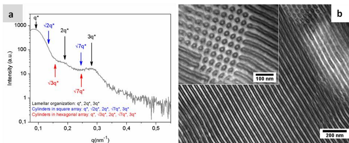
Figure 2. a) SAXS profiles of SBM films cast from CHCl 3 with three possible indexations: lamellae, cylinders in hexagonal or square array. b) Cylinder stacking of SBM observed by TEM. The B block is stained in black, the S block in light grey by OsO 4 vapor. 41
