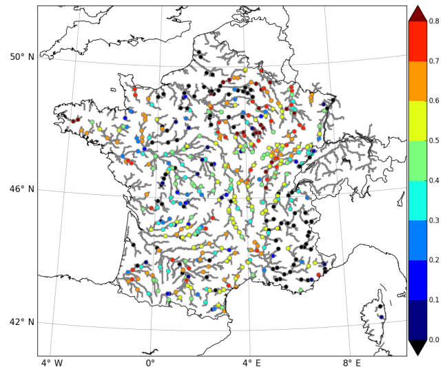
Figure 2. Nash efficiency scores for each station over France for the NIT simulation, calculated over the period 2007–2014. The river network is also shown.
