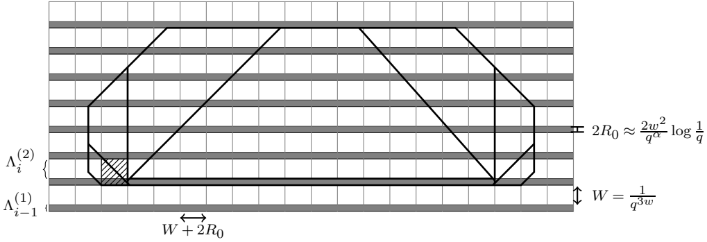
Fig 11: The partition of \Lambda into strips \Lambda_i = \Lambda_i^{(1)} \cup \Lambda_i^{(2)} , i \in [M] . The hatched region represents a square Q_{i,j} , which we would like to resample. The thick polygon is the snail V with its trapezoids. Note that its base B does not intersect Q_{i,j} and (almost) spans the squares Q_{i,j+1}, \dots, Q_{i,j+\lambda} .
