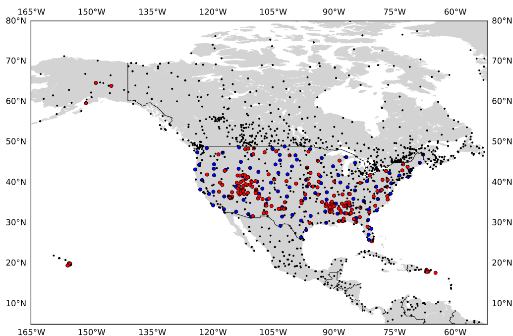
Figure 1. Region under study. Overlapped are the observations from the SYNOP network (black dots), and the ground soil moisture observations from the SCAN (red circles) and USCRN (blue circles) networks in the US.
