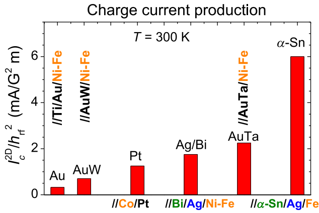
FIG. 1. Ratio between charge current production and h_{\text{rf}}^2 (where h_{\text{rf}} is the magnetic rf field) by ISHE (Au [25], Pt [19], \text{Au}_{0.97}\text{W}_{0.07} [25], \text{Au}_{0.975}\text{Ta}_{0.025} [26]) or IEE (Ag/Bi [5] and Ag/ \alpha -Sn [9]) in experiments of spin pumping ferromagnetic resonance at room temperature. The results are obtained in the same setup ( f \sim 9.7 GHz) and with the same geometry (i.e., width of 0.4 mm). The definitely larger experimental production with the \alpha -Sn TI is in reasonable agreement with the calculated gain results in Table I (if normalized by the injected spin current, the advantage of \alpha -Sn is even larger). We should point out that j_c^{2D}/h_{\text{rf}}^2 depends not only on the intrinsic parameters of the spin-orbit coupling material, \theta_{\text{SHE}} , \lambda_{\text{SF}} , \lambda_{\text{IEE}} , but also on extrinsic parameters such as interface parameters throughout the whole stack.
