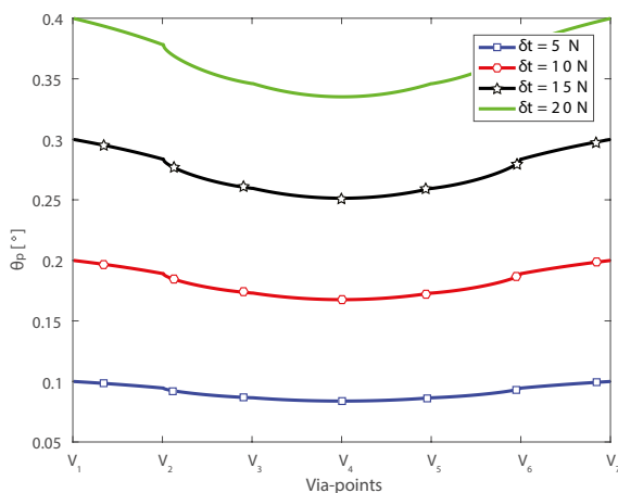
Fig. 6: Parasitic inclination \theta_p of the moving-platform for different values of the cable tension difference \delta t into the cable-loop
