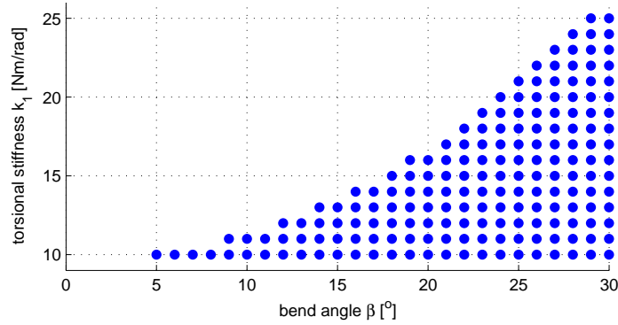
Fig. 5. Effects of the driving shaft stiffness k_1 and bend angle \beta onto the dynamic torsional stability with speed \Omega_0 = 19\pi rad/s.
