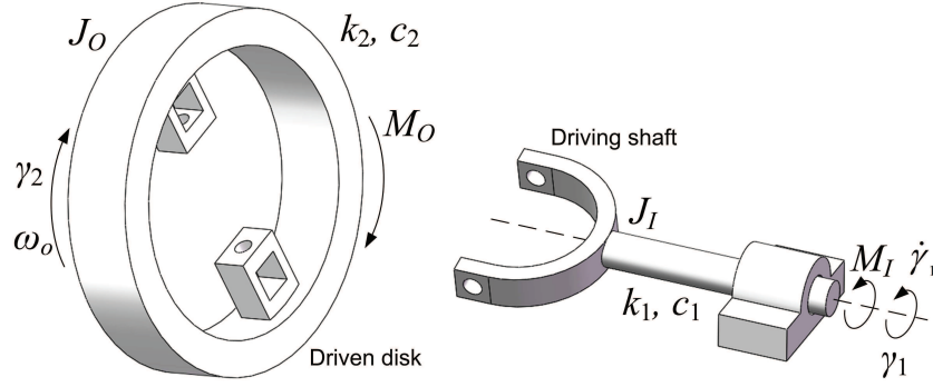
Fig. 3. The driving and driven parts of the U-joint mechanism.
