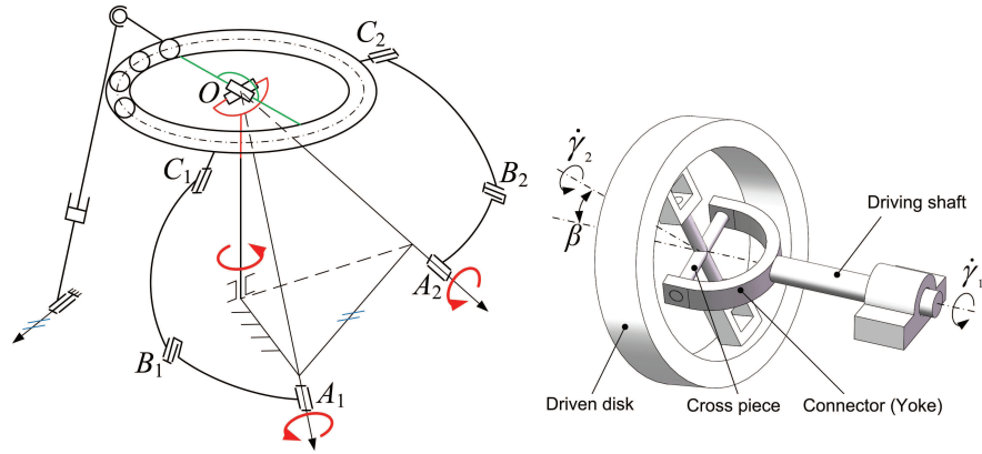
Fig. 2. Kinematic architectures of the wrist mechanism and its U joint.
