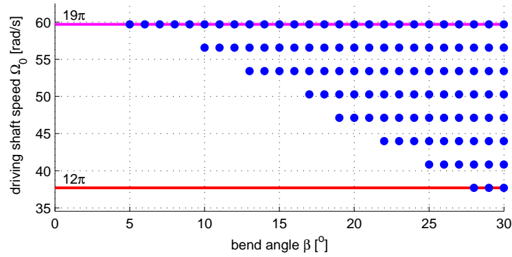
Fig. 4. Effects of the driving shaft speed \Omega_0 and bend angle \beta onto the torsional stability of the parallel wrist with stiffness k_1 = 10 Nm/rad (blue point means torsional dynamic instability).
