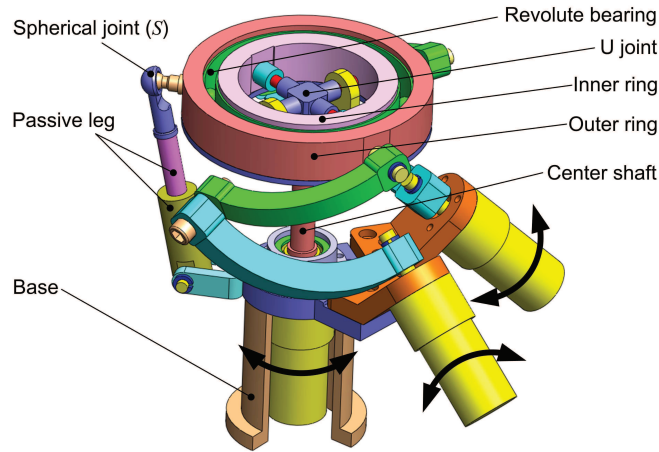
Fig. 1. CAD model of the parallel wrist mechanism.
