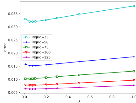
Figure 17: Influence of the grid resolution on the relative L_2 error of v , for the flow between two cylinders (VP MRT LBM, \tau = 0.7 ).
