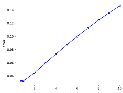
Figure 11: Influence of \tau on the relative L_2 error of v , for the flow between two cylinders (VP SRT LBM).
