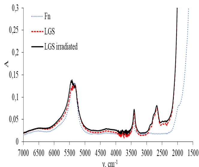
Figure 5: Comparison between IR absorption spectra of LGT 'Fn', LGS and irradiated LGS samples.
