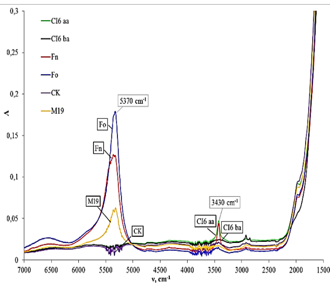
Figure 3: IR absorption spectra of LGT samples.
