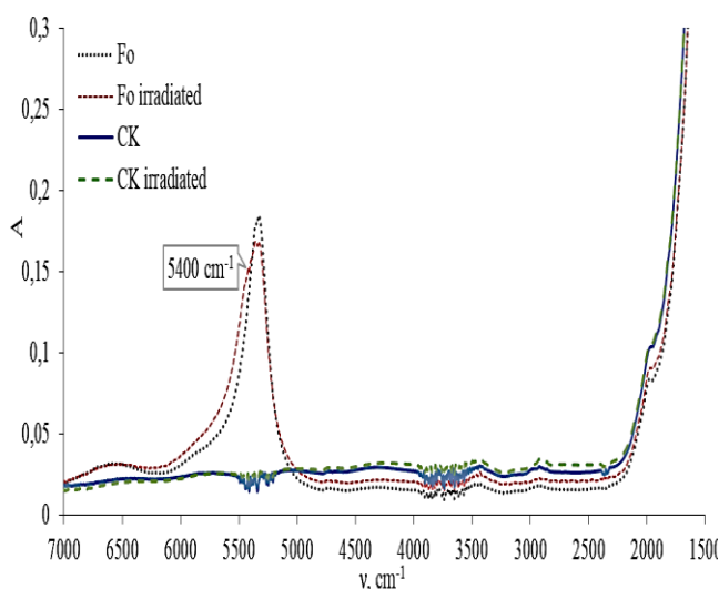
Figure 4: Ultraviolet irradiation effect on IR absorption spectra of LGT samples 'Fo' and 'CK'.
