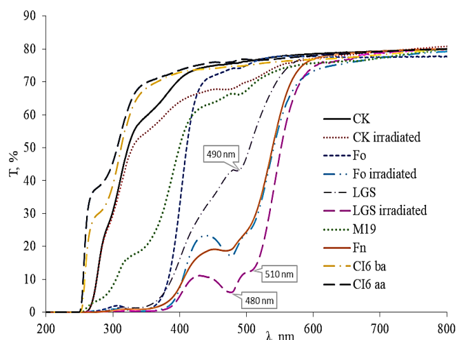
Figure 2: UV-Vis transmission spectra of LGT and LGS samples.
