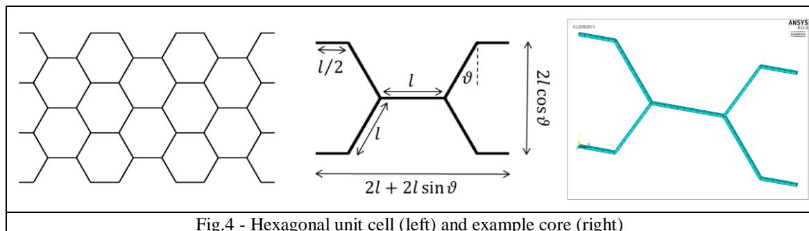
Fig.4 - Hexagonal unit cell (left) and example core (right)
