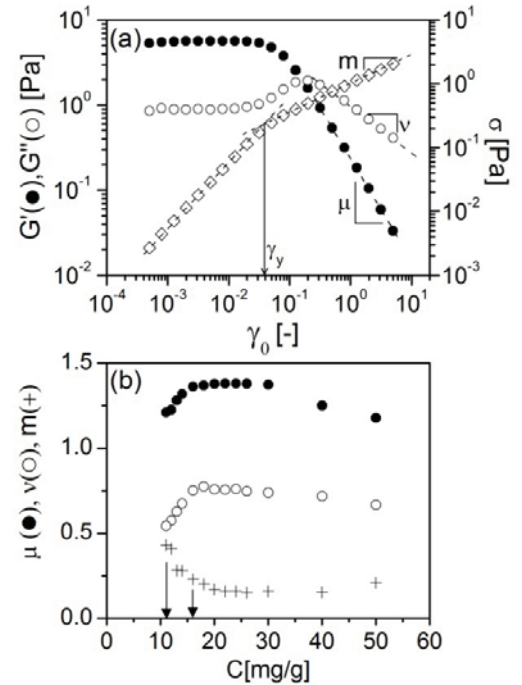
Fig. 4 (a) Dynamic strain sweep at \omega = 1 rad/s of the microgel suspension with C = 11 mg/g; \mu , \nu , and m are the exponents of the power law variations for the storage modulus (●), loss modulus (○) and shear stress (□) at large strains. (b) Variations of \mu (●), \nu (○), and m (+) versus polymer concentration; the arrows point to the entropic glass ( C_G \approx 11 mg/g) and jammed glass ( C_J \approx 16 mg/g) transitions as explained in the text.
