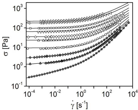
Fig. 7 Flow curves of entropic [ C = 12 ( \oplus ), 13 ( \triangle ), and 14 ( \diamond ) mg/g] and jammed glasses [ C = 16 ( \circ ), 18 ( \triangle ), 20 ( \diamond ), 24 ( \nabla ), 30 ( \square ), 40 ( \langle ), 50 ( \triangleright ) mg/g]. Lines are fits of the data to Eq. 2 ( C_G < C < C_J ) and Eq. 3 ( C > C_J ).
