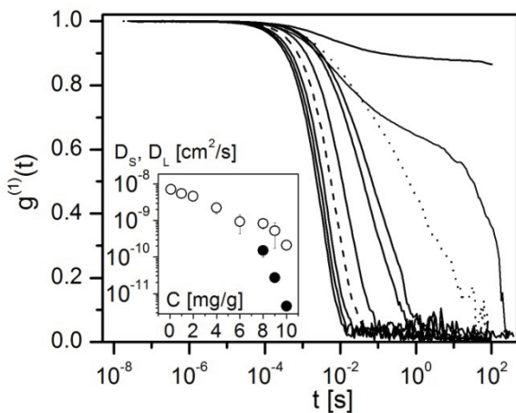
Fig. 1 Ensemble-averaged field autocorrelation functions for suspensions with C = 12, 11, 10 (....), 9, 8, 6, 4 (- - -), 2, 1, 0.1 mg/g (from right to left) at q = 0.021 nm -1 ( qR_h \cong 6 ). The inset shows the variations of the short (○) and long (●) time self-diffusion coefficients, D_s and D_L , measured for qR_h > 6 .
