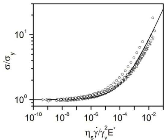
Fig. 8 Master curve obtained by plotting the flow curves measured in the jammed regime (Fig. 7) in the set of coordinates derived from the elasto-hydrodynamic model [ C = 16 ( \circ ), 18 ( \triangle ), 20 ( \diamond ), 22 ( \square ), 24 ( \nabla ), 26 ( + ), 30 ( \square ), 40 ( \langle ), 50 ( \triangleright ) mg/g]. The solid line is the theoretical flow curve expected from the model.
