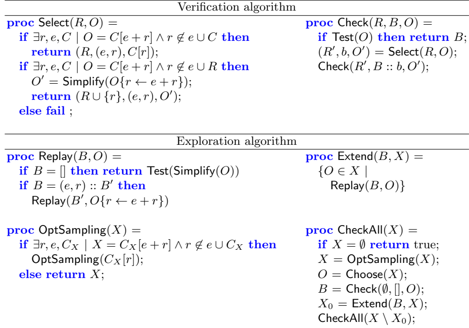
Fig. 5. Verification algorithm for probing security
