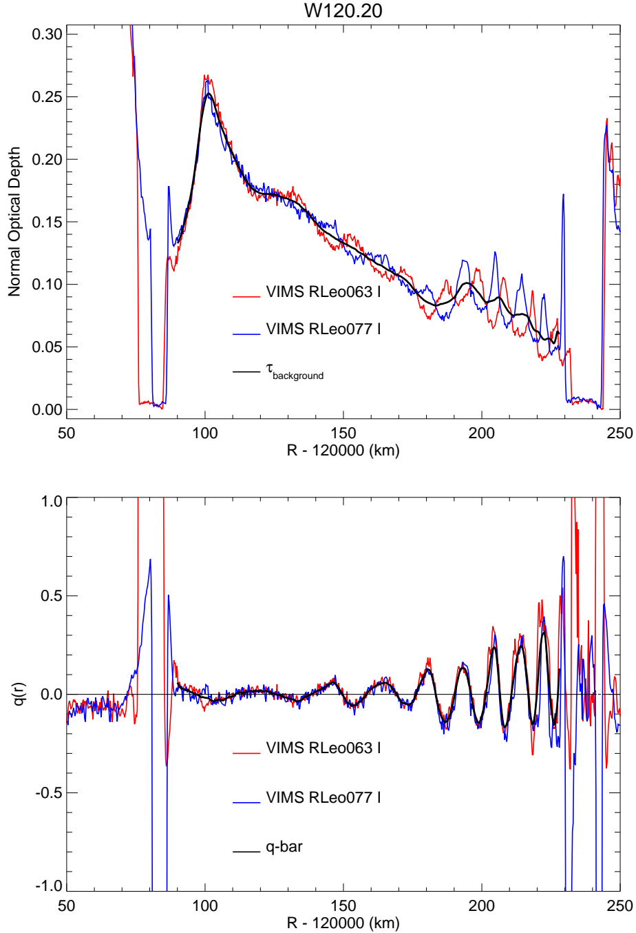
Figure 23. The background optical depth \bar{\tau}(r) (upper panel) and intrinsic radial structure q(r) (lower panel) of standing wave W120.20, from VIMS RLeo063 I and VIMS RLeo077 I radial occultation profiles obtained at nearly opposite phases of the wave. See text for details.
