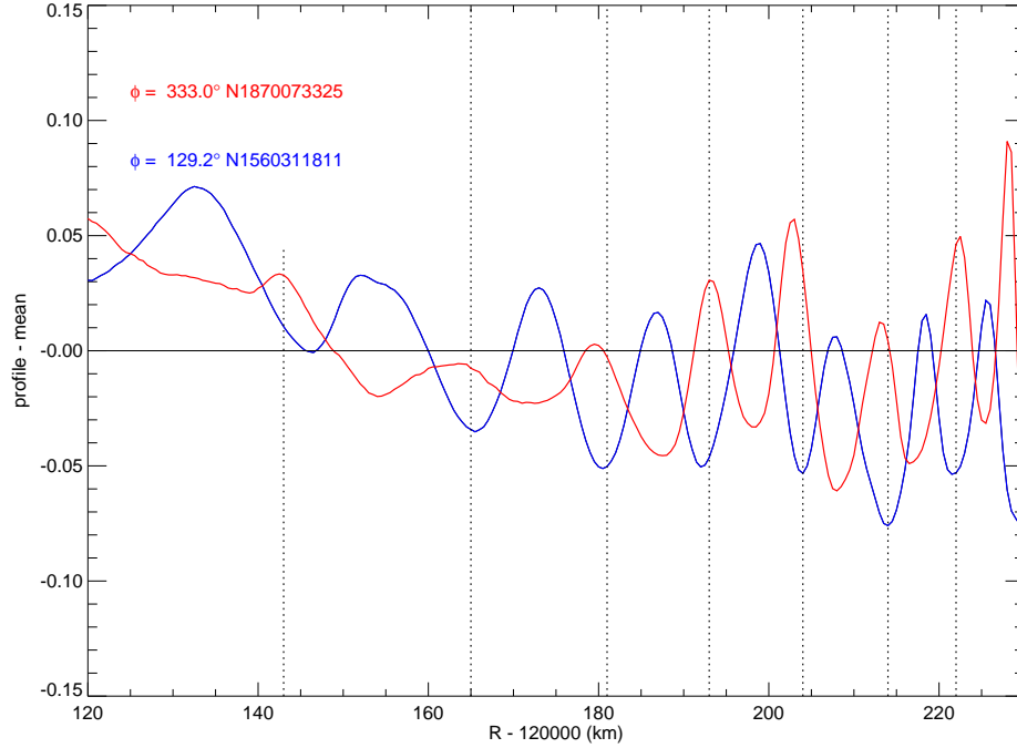
Figure 22. Radial brightness profiles extracted from the pair of ISS images in Fig. 21, after approximate removal of a background gradient. The m = 1 phases of these two wave profiles differ by 156.2^\circ , for an assumed pattern speed \Omega_p = 4.72^\circ \text{ d}^{-1} . The vertical dotted lines are drawn at the set of radii derived from the RSS profiles shown in Figs. 16 and 19, and match the locations of the corresponding peaks for image N1870073325 within a km or so.
