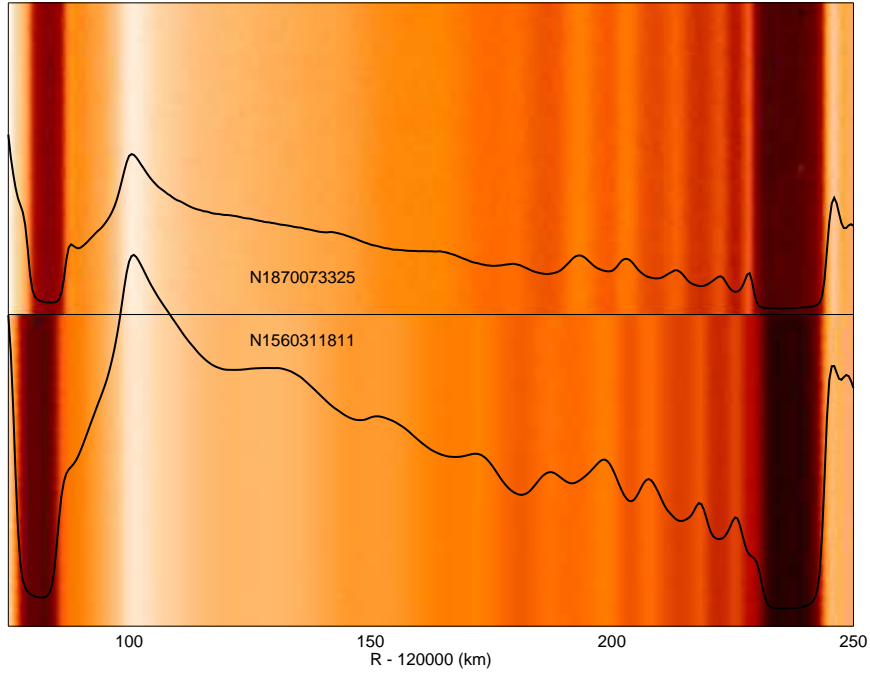
Figure 21. A pair of ISS images of the W120.20 standing wave, reprojected into radius and longitude. At the left edge of the images we see the slightly eccentric outer edges of the Laplace ringlet and gap, while at the right edge we see the eccentric inner edge of the narrow Bessel gap. Superimposed are radial profiles of brightness, averaged in longitude.
