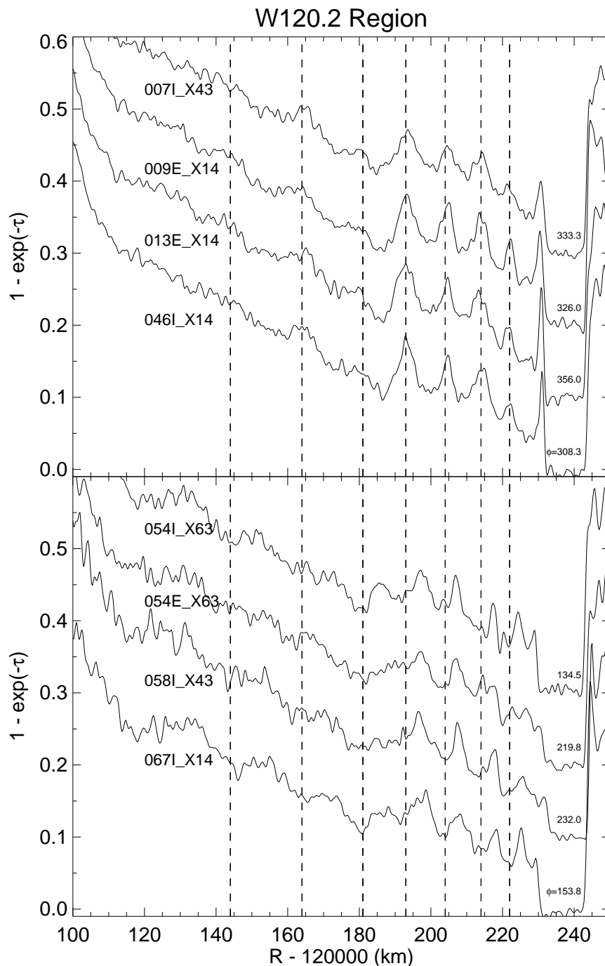
Figure 16. A subset of RSS occultation profiles of the W120.2 region, selected to illustrate the bimodal character of the wave crests and troughs. The profiles are labeled by Cassini rev number, I or E for ingress or egress, and by the RSS wavelength band (X, in all cases shown here) and NASA Deep Space Net station number. Vertical dashed lines indicate the approximate locations of optical depth maxima in the top set of profiles, at 120,000+144, 164, 181, 193, 204, 214 and 222 km, each of which roughly corresponds to a minimum in optical depth in the lower set of profiles. The phase \phi of each profile (cf. Eq. 18) is labeled at lower right.
