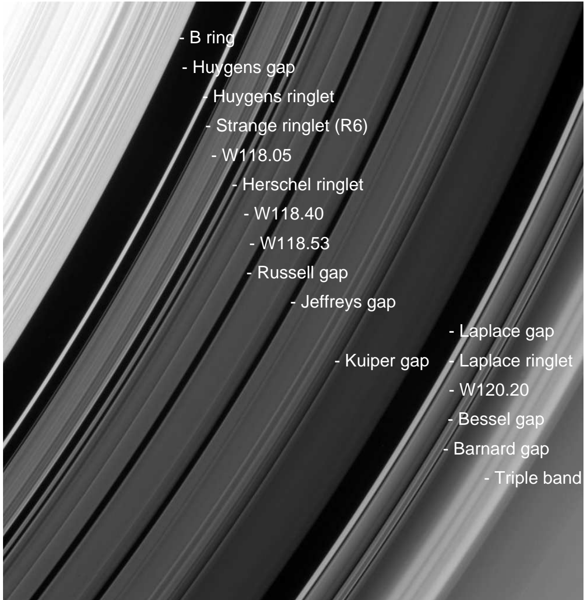
Figure 1. An overview of the Cassini Division with its named gaps and ringlets, from Cassini image N1495286873 (taken on 2005 May 20). The four waves that are the subject of this investigation are identified as W118.05, W118.40, W118.53 and W120.20. The projected ring plane resolution of the image is 4 km/pixel and the observer ring elevation is -21.6^\circ .
