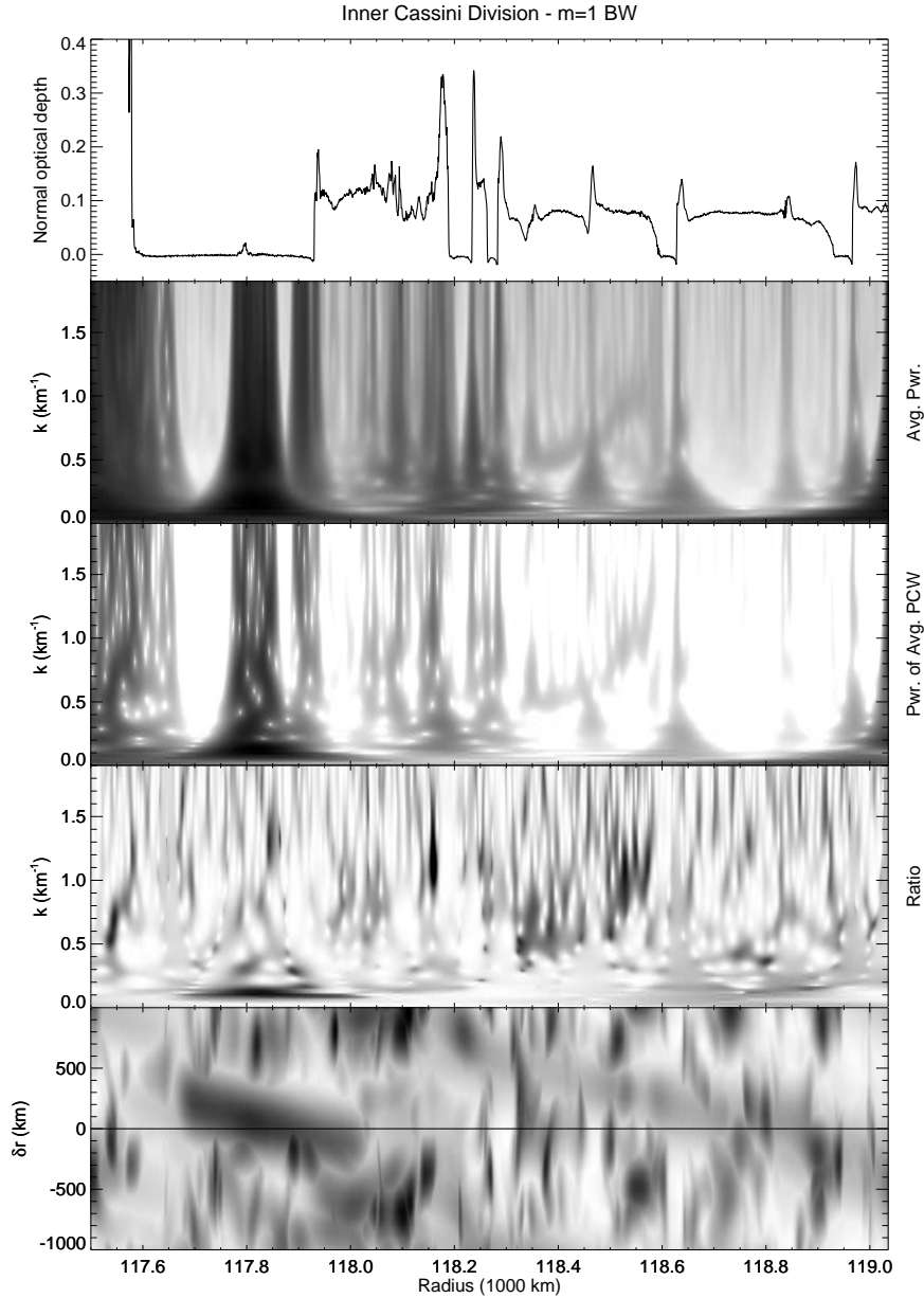
Figure 13. Phase-corrected wavelet analysis for Bands 1 and 2, assuming that the structure is due to bending waves with m = 1 and \Omega_p \simeq \dot{\Omega}_{\text{sec}} . The format is the same as that of Fig. 6, except that the 6th panel is omitted here. No clear bending wave signals are seen, except the power at low wavenumbers between 117,700 and 117,950 km, which is likely due to the inclined Strange (R6) ringlet.
