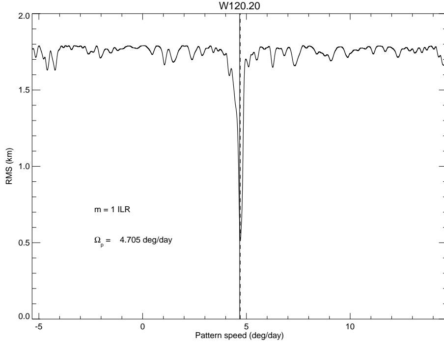
Figure 18. RMS radius residuals for an elliptical ( i.e. , m = 1 ) fit to the single wave crest in W120.20 with a mean radius of 120,206 km, assuming an m = 1 pattern and plotted as function of the assumed pattern speed \Omega_p . For this fit we used only the RSS profiles shown in Fig. 5. The best-fitting ellipse has an amplitude ae = 2.2 km and a pattern speed of 4.705^\circ \text{ d}^{-1} .
