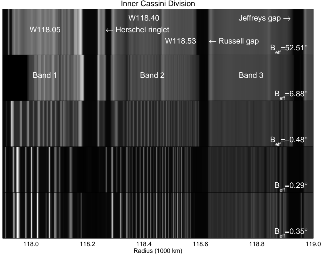
Figure 14. Five Cassini ISS narrow angle camera images of the inner Cassini Division, reprojected at a uniform scale into radius and longitude. The effective ring opening angle B_{\text{eff}} is labeled at right for each image; see Table 1 for a list of image numbers and additional geometric parameters. Visible from left to right are the outer Huygens gap edge (except in the 2nd image), the Herschel gap and ringlet, the Russell gap and the Jeffreys gap. Bounded by these gaps are Bands 1, 2 and 3 of Flynn and Cuzzi (1989). The wave structures in Bands 1 and 2 are especially prominent in the lower three images (see text).
