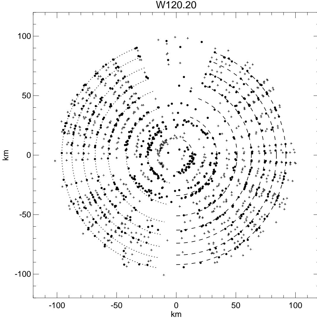
Figure 19. A polar projection (r, \phi_{\lambda,t}) of the measured locations of wave crests and troughs for the wave W120.20 in the outer Cassini Division, as seen in a frame rotating at a uniform rate of \Omega_p = 4.72^\circ \text{ d}^{-1} , with the origin at a radius of 120,130 km and the positive x-axis corresponding to \phi_{\lambda,t} = 0 (the phase at which the wave maxima reach their highest amplitude). In this coordinate system, the azimuthal nodes in the pattern of maxima and minima are oriented vertically. Filled circles indicate optical depth maxima, while crosses indicate the intervening minima. The dashed circular arcs are drawn at the same set of radii shown in Fig. 16, from 120,144 to 120,222 km, and match the optical depth maxima on the right side of the diagram. Dotted circular arcs indicate radii midway between the dashed circular arcs, and match the optical depth maxima on the left side of the diagram.
