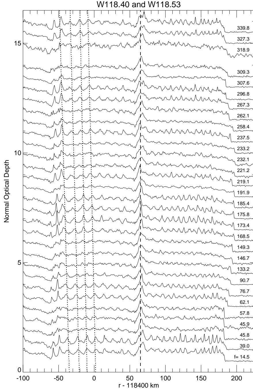
Figure 4. Optical depth profiles of waves W118.40 and W118.53 in Band 2, offset vertically for clarity and sorted by true anomaly f (labeled at right) for an assumed pattern speed of 4.950^\circ \text{ d}^{-1} . The data are from X-band RSS occultations on revs 7 – 67, processed at a radial resolution of 1 km. The eccentric inner edge of the Russell gap, with a radial amplitude ae = 7.6 km, is seen at the extreme right edge of the plot. The slanted dotted lines approximately trace the trend of decreasing radius with increasing true anomaly of several wavecrests in the inner region of W118.40. Visible as a narrow peak in optical depth separating the two wave regions is the Pan 6:5 ILR density wave at \sim 118,465 km, marked by a vertical dashed line.
