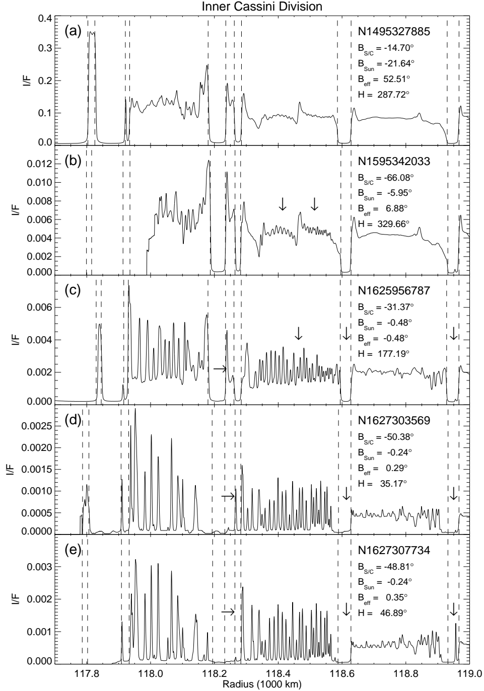
Figure 15. Radial scans of the ISS NAC images shown in Fig. 14. See Table 1 for a list of image numbers and geometric parameters. Visible from left to right are the Huygens ringlet and outer gap edge, the Herschel gap and ringlet, the Russell gap and the Jeffreys gap. Vertical dashed lines correspond to the predicted apparent radius of sharp-edged features, taking account of their possibly non-circular and/or inclined orbital shapes. The wave structures W118.05, W118.40 and W118.53 are especially prominent in the lower three profiles (see text). Arrows highlight the changing features noted in the text.
