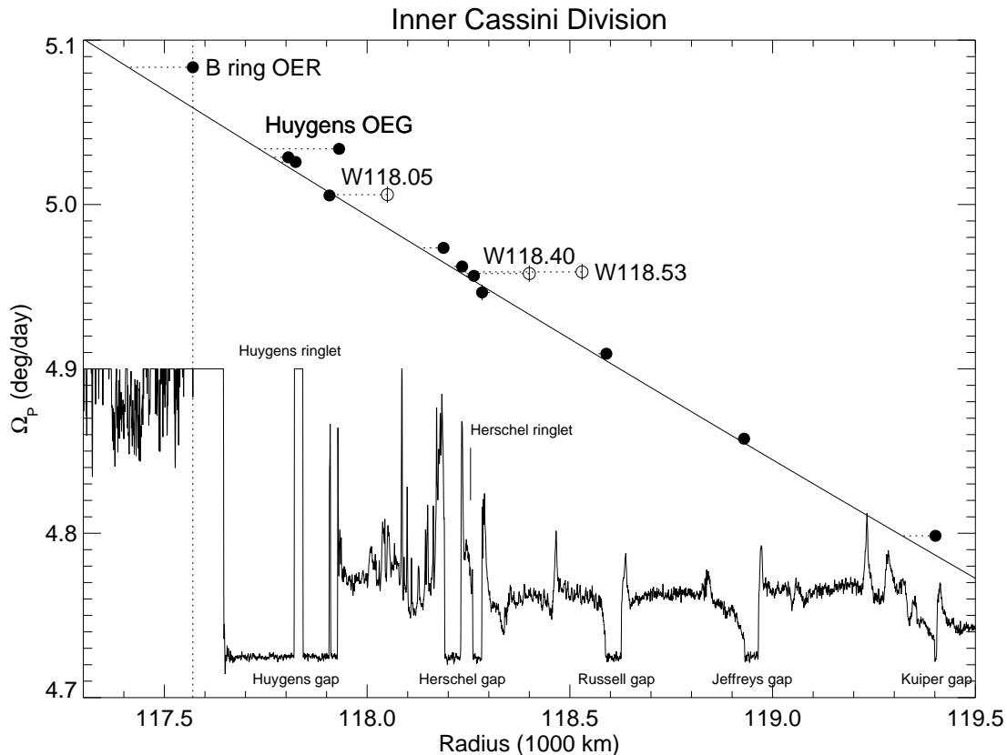
Figure 9. Regional m = 1 pattern speeds in the inner Cassini Division. Filled circles denote gap and ringlet edges from French et al. (2016a) while open circles show the waves discussed in this paper. The diagonal line shows the apsidal precession rate \dot{\omega}_{\text{sec}} calculated from Saturn’s zonal gravity harmonics. Horizontal dotted lines connect the measured pattern speeds for the gaps or ringlets and waves to their corresponding resonant radii. The vertical dotted line at 117570.12 km marks the mean radius of the outer edge of the B ring, from Table 4 of Nicholson et al. (2014a).
