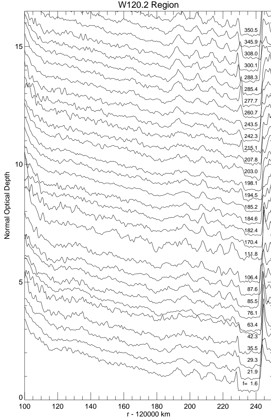
Figure 5. Optical depth profiles of wave W120.20 in the outer Cassini Division, offset vertically for clarity and sorted by true anomaly f (labeled at right) for an assumed pattern speed of 4.720^\circ \text{ d}^{-1} . The data are from X-band RSS occultations on revs 7 – 67, again processed at a radial resolution of 1 km. The Bessel gap and its eccentric inner edge, with a radial amplitude of ae = 1.8 \text{ km} , is seen at the right edge of the plot.
