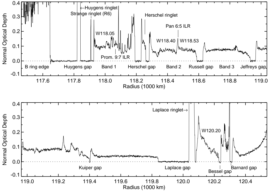
Figure 2. Prominent ringlets and gaps in the Cassini Division, as seen in an optical depth profile from the Cassini RSS egress occultation on rev 7. The wave features that are the focus of this work are illustrated: W118.05, W118.40, W118.53, and W120.20. The data are shown at a radial processing resolution of 1 km.
