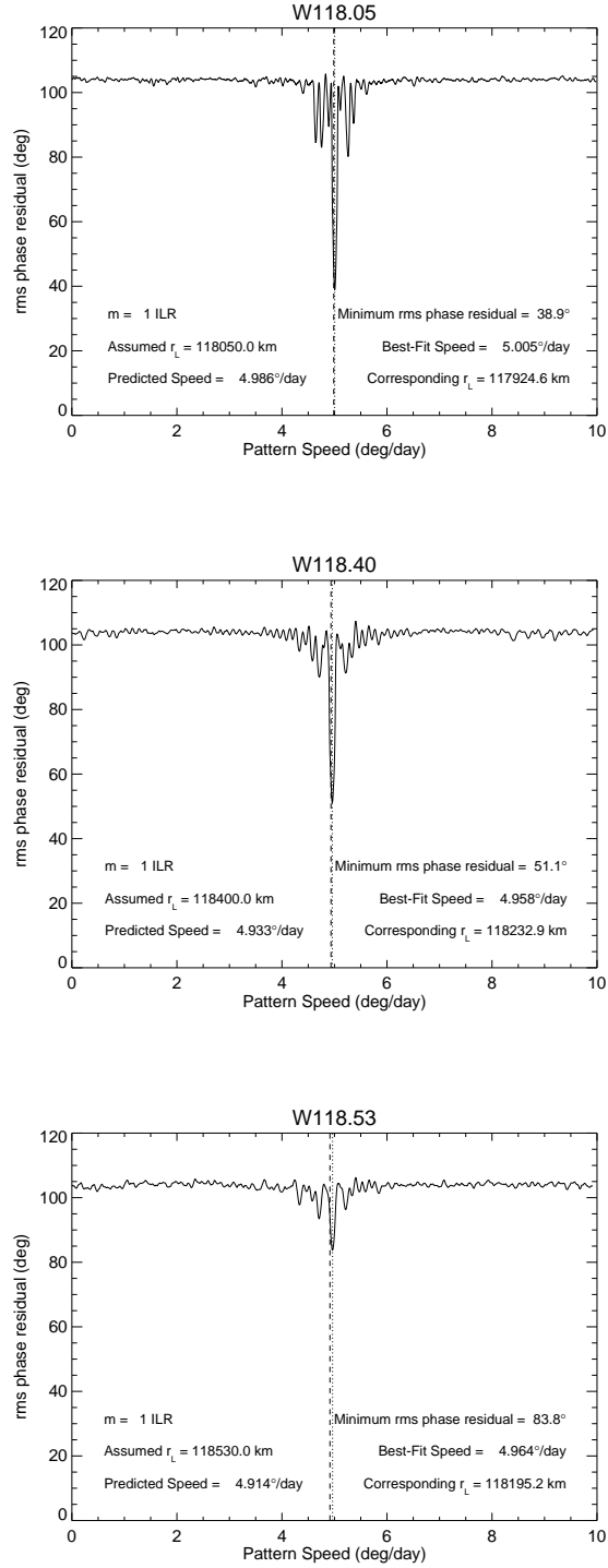
Figure 7. Pattern speed scans for waves W118.05, W118.40 and W118.53 for m = 1 , based on comparing the observed and predicted phase differences between pairs of occultations (see text for details). The data set includes all VIMS and RSS occultations, subject to signal-to-noise limitations. For each wave, the best-fitting pattern speed (indicated by the vertical dotted line) and corresponding resonant radius are listed, along with the minimum RMS phase residual. Also listed are the predicted values of \Omega_p used to center our search region, indicated by the vertical dashed line.
