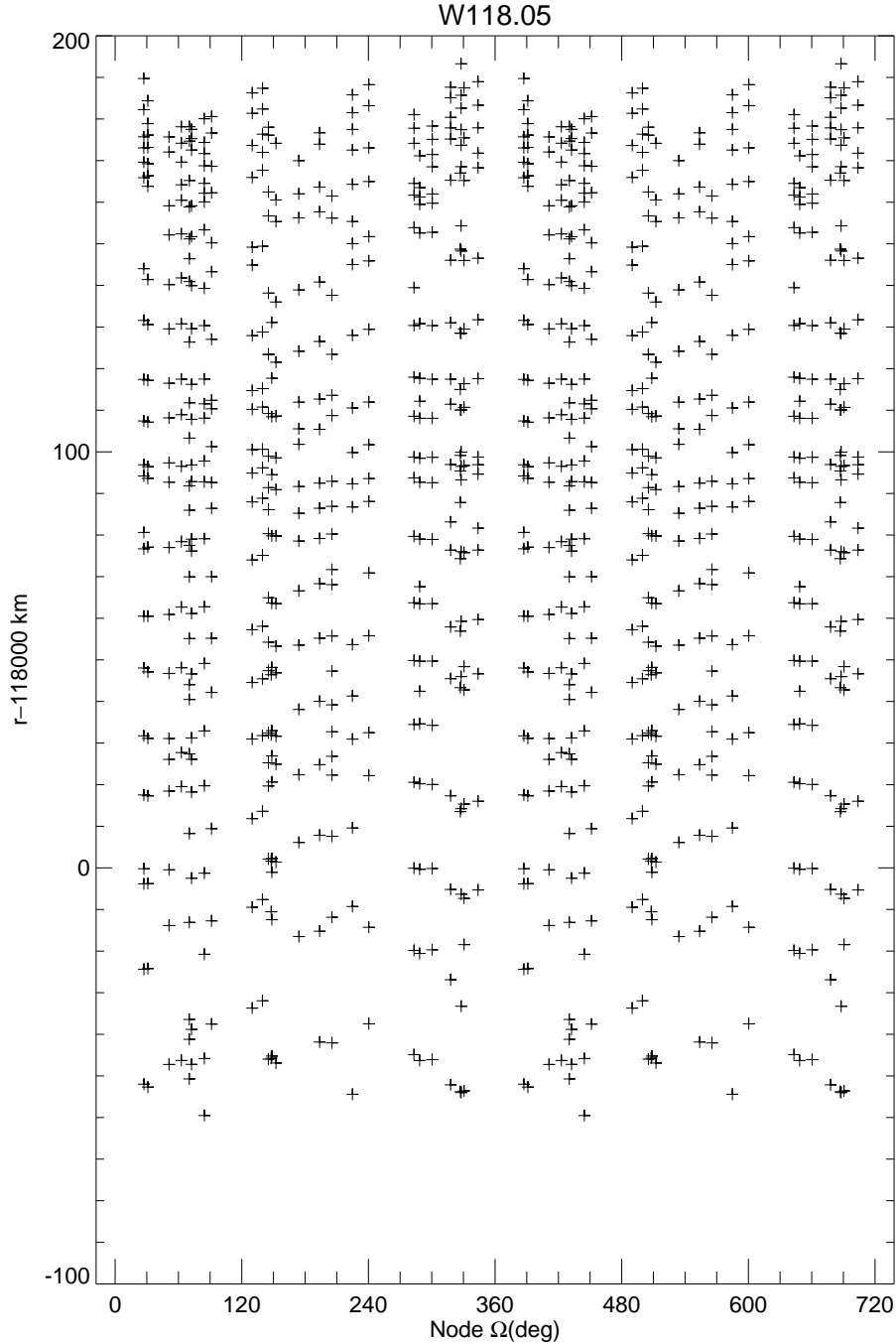
Figure 12. Successive wave crest locations for RSS observations of wave W118.05 in Band 1 as in Fig. 8, but plotted as a function of ascending node \Omega . There is no clear organized behavior to indicate that this is a bending wave.
