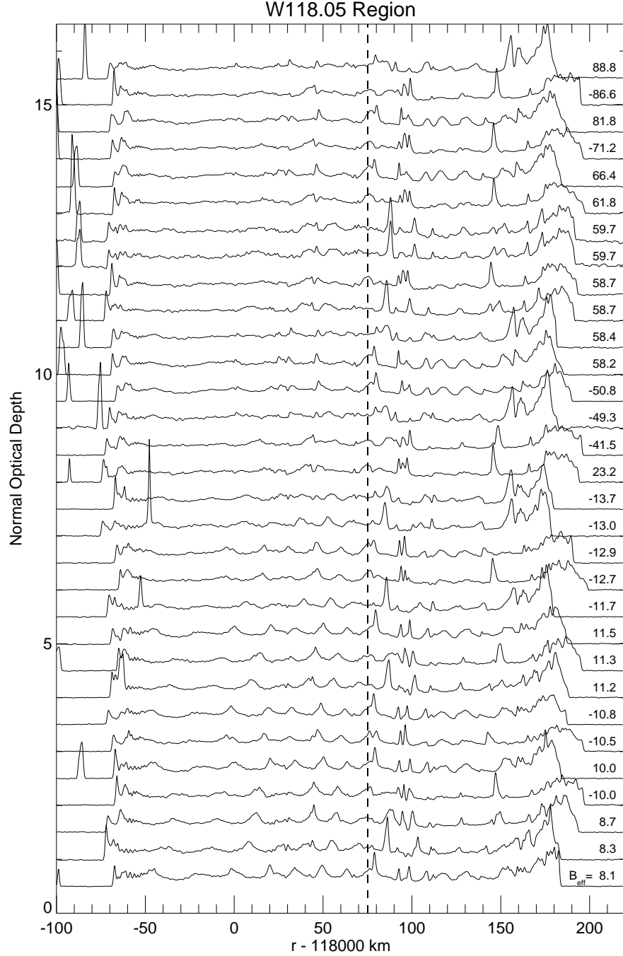
Figure 10. Profiles of wave region W118.05 in Band 1, sorted by the absolute value of B_{\text{eff}} . The data are the same as the RSS occultation profiles shown in Fig. 3. The vertical dashed line marks the Prometheus 9:7 ILR.
