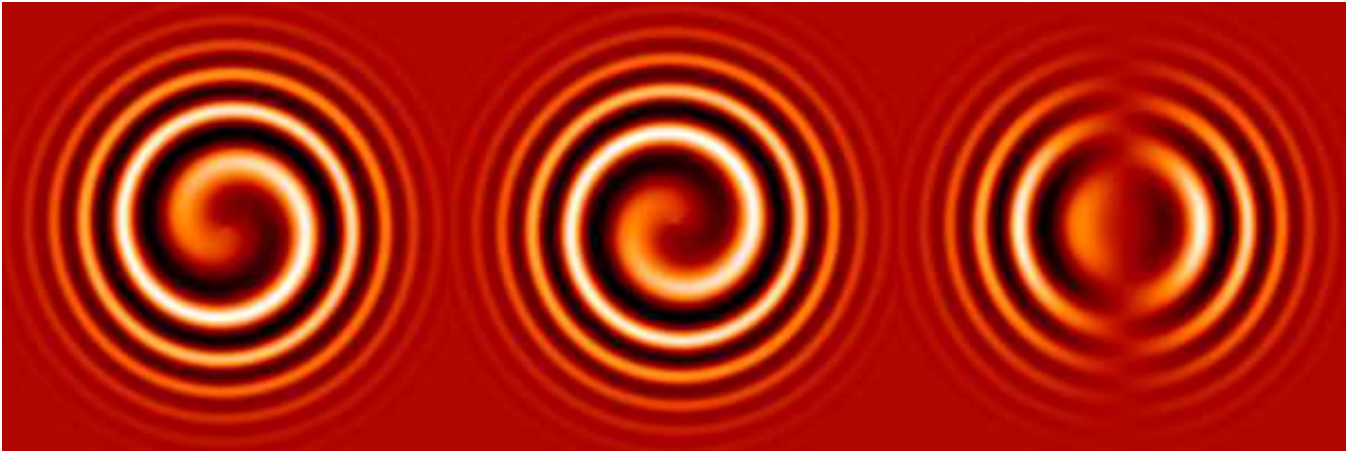
Figure 20. A single three-panel frame from a movie illustrating the decomposition of the standing wave W120.20 into leading and trailing spiral density waves. The left panel shows a trailing spiral wave with m = 1 , while the middle panel shows a leading m = 1 spiral with the same amplitude and resonant radius. The right panel shows the standing wave that results from adding the leading and trailing waves. In inertial space, all three waves rotate counter-clockwise at the pattern speed \Omega_p = 4.72^\circ \text{ d}^{-1} . The spiral waveforms are standard linear density waves, following the model of Shu (1984), with an artificial viscous damping term added. Compare the right panel with the measured peak and trough locations for wave W120.2 in Fig. 19. The complete movie is contained in the Supplementary Material.
