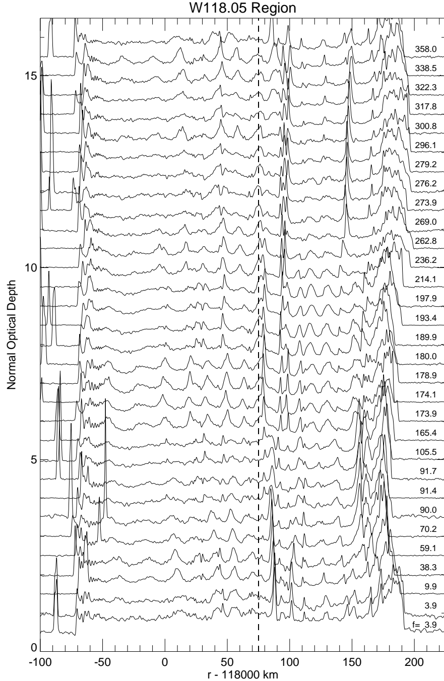
Figure 3. Optical depth profiles of wave W118.05 in Band 1, offset vertically for clarity and sorted by true anomaly f (labeled at right) for an assumed pattern speed of 5.000^\circ \text{ d}^{-1} . The data are from X-band RSS occultations on revs 7 – 67, processed at a radial resolution of 1 km. The narrow R6 (or Strange) ringlet and the outer edge of the Huygens gap are seen at the left edge of the plot, while the eccentric inner edge of the Herschel gap is seen at the right edge. The latter has a substantial radial amplitude of ae = 8.3 km. Only barely visible at this scale and resolution is the weak Prometheus 9:7 ILR density wave outward of its resonance radius of \sim 118,075 km, marked by a vertical dashed line.
