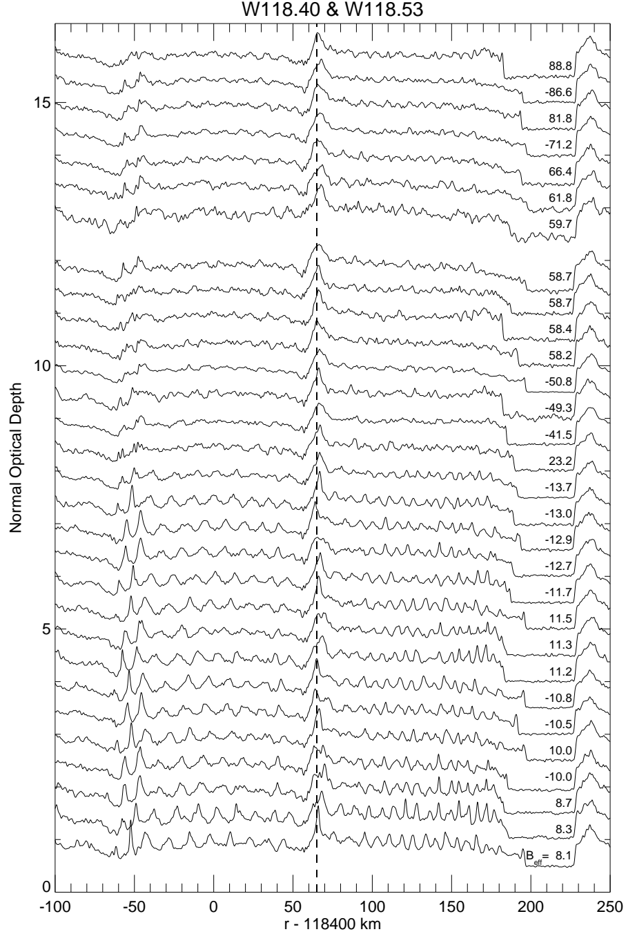
Figure 11. Profiles of waves W118.40 and W118.53 in Band 2, sorted by the absolute value of B_{\text{eff}} . The data are the same as the RSS occultation profiles shown in Fig. 4. The vertical dashed line marks the Pan 6:5 ILR.
