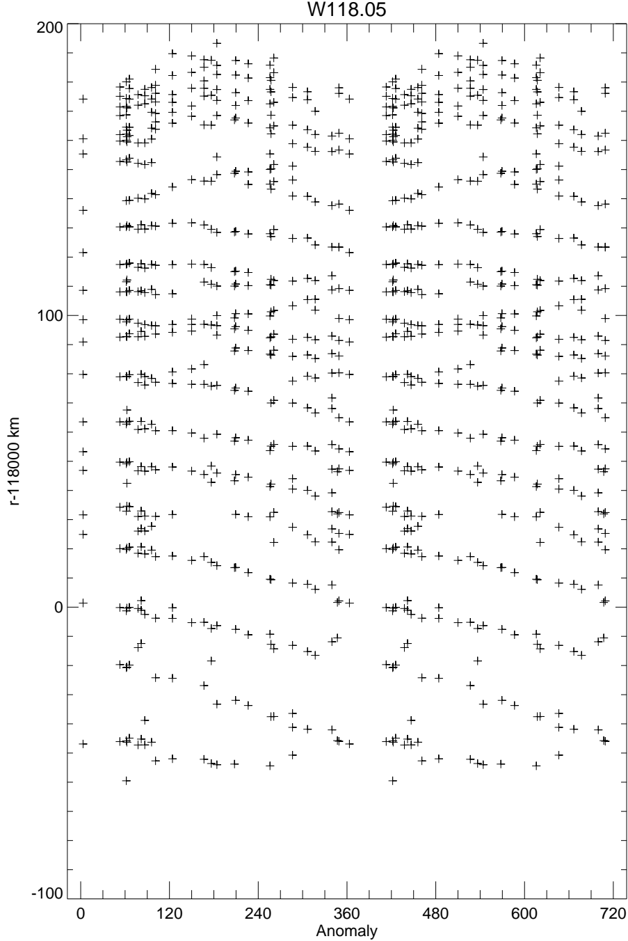
Figure 8. Successive wave crest locations for RSS observations of wave W118.05 in Band 1, as functions of true anomaly f . Series of points for which the radius decreases with increasing f correspond to a trailing spiral pattern, whereas points for which the radius increases with increasing f correspond to a leading spiral. Both types of spiral are seen here, but the trailing spiral is dominant interior to 118,090 km. Note that two full cycles of true anomaly are shown, in order to demonstrate that, in most cases, each arm of the trailing spiral pattern connects smoothly to the next one further inwards, as expected for an m = 1 spiral. A total of 11 or 12 circuits of the trailing spiral are visible here, beginning at a radius of \sim 117,950 km. The inferred resonant radius is 117,920 \pm 35 km.
