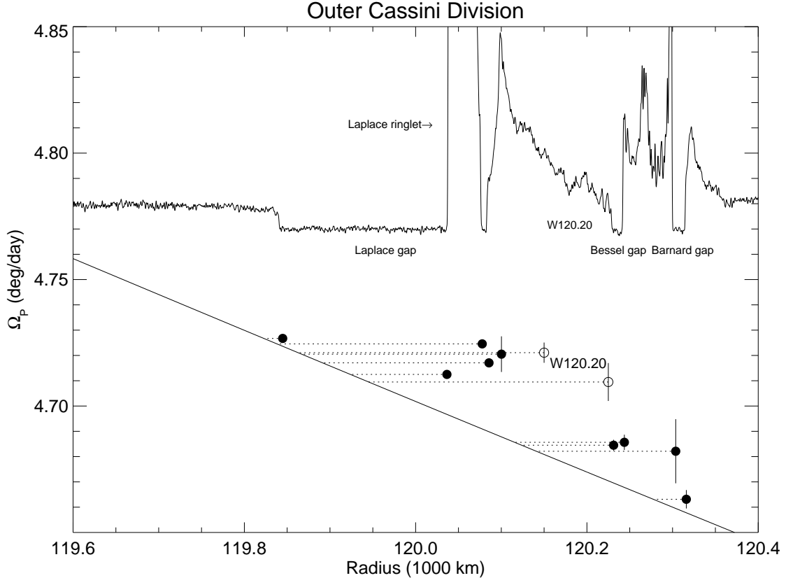
Figure 24. Regional m = 1 pattern speeds in the outer Cassini Division. Filled circles denote gap and ringlet edges from French et al. (2016a) while open circles show the inner and outer portions of the W120.20 wave discussed in this paper. The diagonal line shows the apsidal precession rate \dot{\omega}_{\text{sec}} calculated from Saturn’s zonal gravity harmonics. Horizontal dotted lines connect the measured pattern speeds for the gap or ringlet edges and waves to their corresponding resonant radii.
