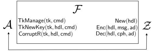
Figure 8: Diagram of the UC-style ideal functionality.
