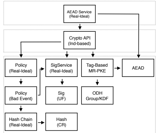
Figure 1: Structure of the machine-checked proof
