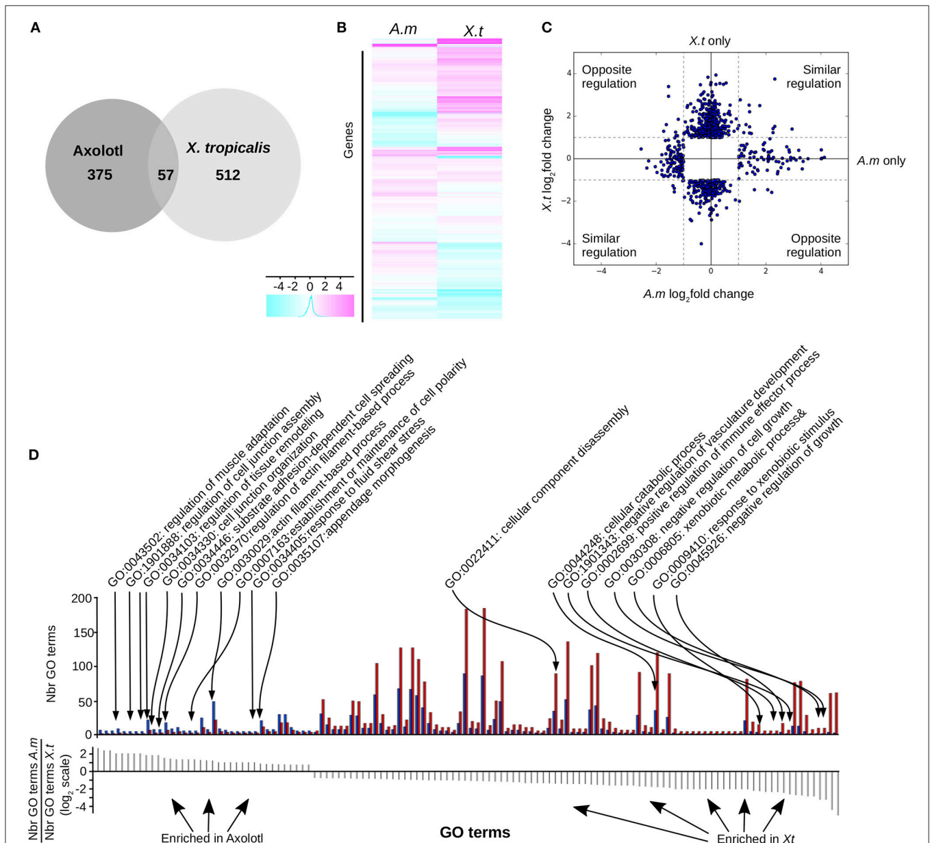
FIGURE 3 | T 3 regulates different gene sets in Axolotl and X. tropicalis at the post-embryonic transition. (A) Overlap between differentially expressed genes in both species. (B) Heatmap of differentially expressed genes in Axolotl (A.m) and X. tropicalis (X.t). (C) Log 2 ratio of TH-induced gene expression changes. (D) Gene ontology analysis. Top: Number of genes for each GO term (not shown), on both species. Blue: Number (Nbr) of terms found in Axolotl. Red: Number of terms found in X. tropicalis . Bottom: ratio of the number of terms found in both species for each GO term (in the same order as the top panel). Positive and negative values correspond to terms mostly found in Axolotl or X. tropicalis gene set, respectively.
