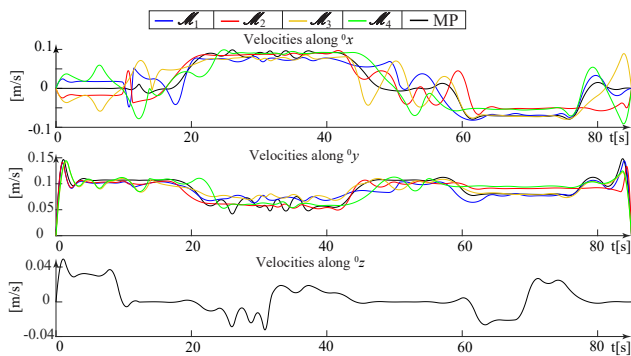
Fig. 4. MoPICK velocity profiles
