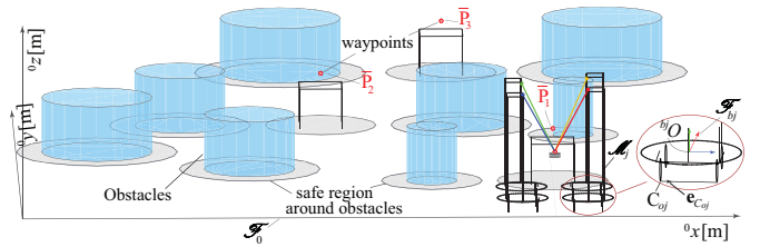
Fig. 2. Test scenario and illustrated environment for the MCDPR.
