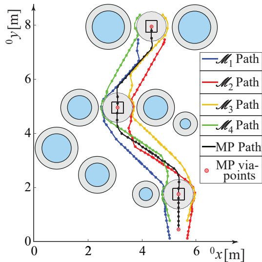
Fig. 3. MoPICK path from direct transcription method.
