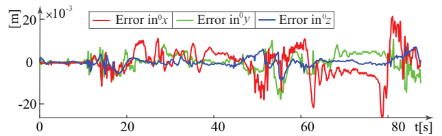
Fig. 6. Error between the actual and the desired moving platform position
