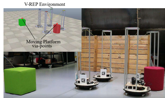
Fig. 7. Simulation and experimental validation on the second scenario
