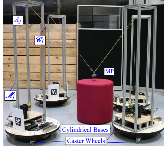
Fig. 1. MoPICK a MCDPR prototype. MoPICK is capable of performing multiple manipulation tasks in a constrained environment, for example, a workshop.
