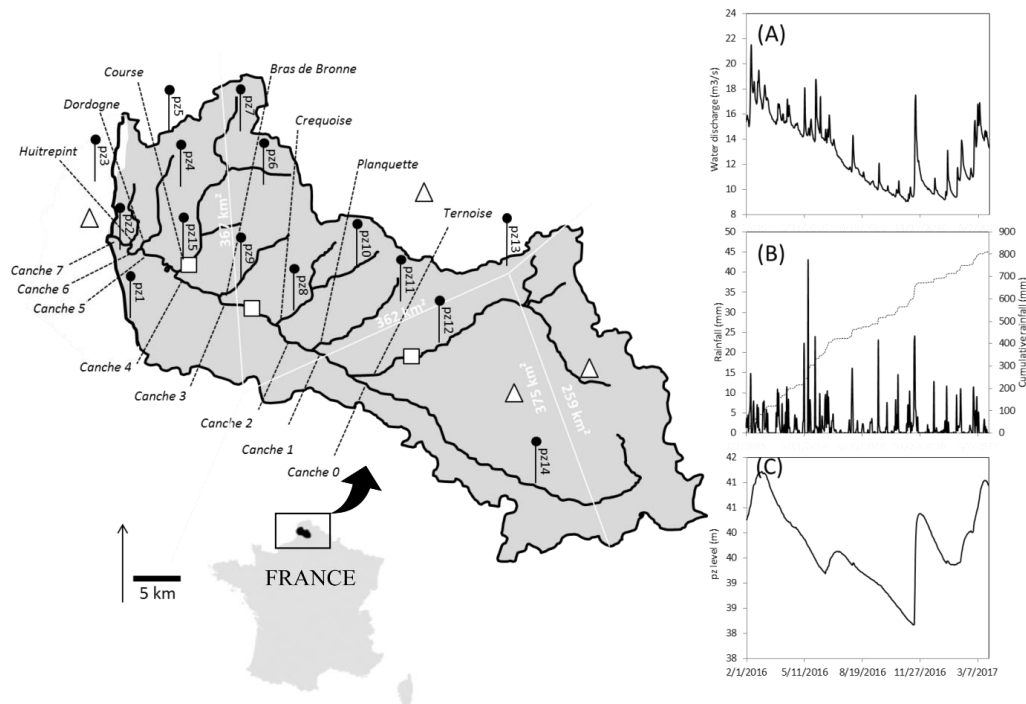
Figure 1. Map of the study area with the Canche River and its main tributaries. Dashed lines point to surface water sampling locations and filled black circles denote ground water sampling locations. The positions of rainfall gauges and discharge gauges are shown as triangle and square markers, respectively. White lines refer to the boundaries between Thiessen polygons used to determine the average rainfall on the catchment. (A) Time series of the water discharge ( \text{m}^3 \text{s}^{-1} ) at the gauging station on the main stream (data from Water Agency Artois-Picardie); (B) average rainfall (mm) on the catchment (data from Météo France); and (C) piezometric level (m) at pz 10 (data from Water Agency Artois-Picardie).
