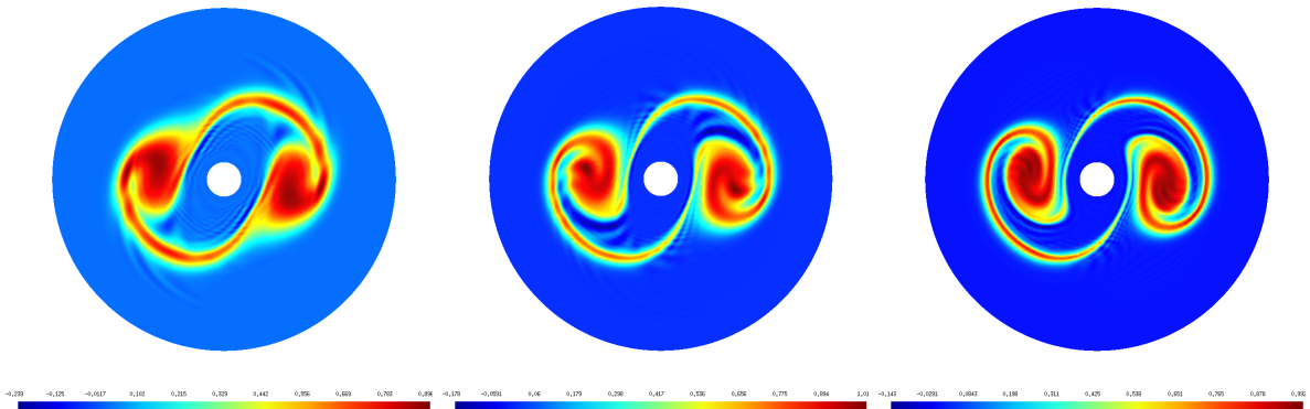
FIGURE 12. (Three-dimensional diocotron test-case) Density at t_{max} = 100 in the poloidal plane \varphi = 0 obtained with n_p = 32 , n_p = 64 and n_p = 128 . Parameters: L = 1 , \lambda_p = 7 , \lambda_t = 3 , DG order p = 2 , \omega = 1.99 .
