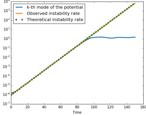
FIGURE 8. (Two-dimensional diocotron test-case) k -th Fourier mode of the potential over time and the instability rate given by the slope of the Fourier mode between t = 20 and t = 60 , compared to the theoretical instability rate. Parameters: \lambda_p = 7 , DG order p = 2 , \Delta t = 0.0125 , \omega = 1.999 .
