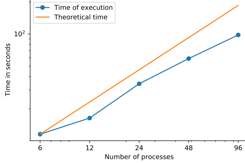
FIGURE 13. (Parallel weak scaling) Time of execution according to the number of MPI processes.
