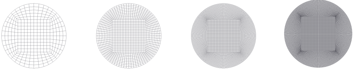
FIGURE 5. Poloidal meshes with refinements n_{\text{raf}} = 5, 10, 20 and 40 . The disk is decomposed into 12 patches and each patch is meshed with n_{\text{raf}}^2 quadrilaterals, where n_{\text{raf}} is the refinement number.
