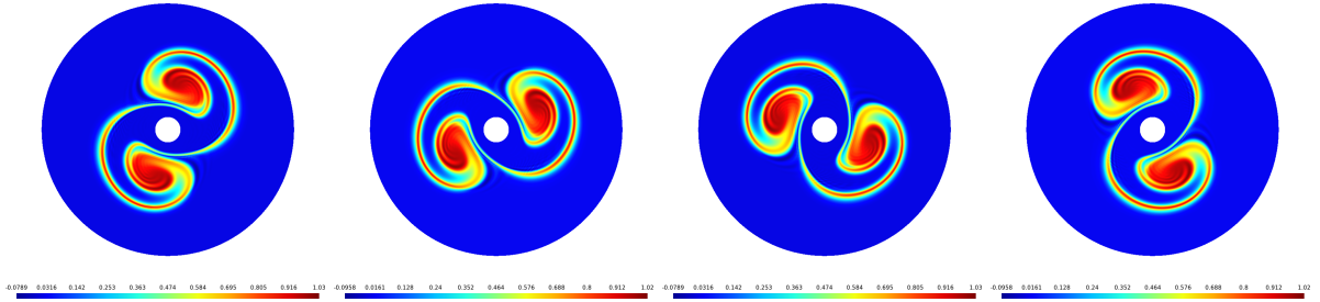
FIGURE 10. (Three-dimensional diocotron test-case) Density at t_{\max} = 100 for the poloidal planes \varphi = 0 , \varphi = \frac{L}{4} , \varphi = \frac{L}{2} and \varphi = \frac{3L}{4} . Parameters: \lambda_p = 7 , \lambda_t = 600 , DG order p = 2 , \omega = 1.99 , n_p = 128 .
