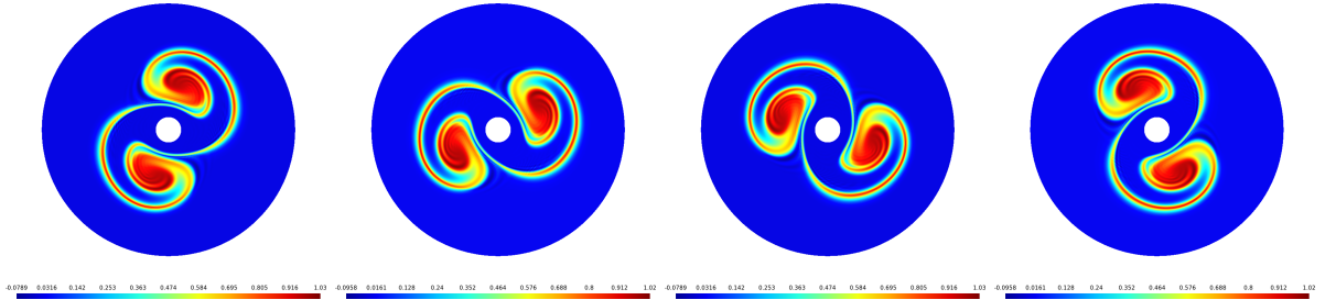
FIGURE 10. (Three-dimensional diocotron test-case) Density at t_{\max} = 100 for the poloidal planes \varphi = 0 , \varphi = \frac{L}{4} , \varphi = \frac{L}{2} and \varphi = \frac{3L}{4} . Parameters: \lambda_p = 7 , \lambda_t = 600 , DG order p = 2 , \omega = 1.99 , n_p = 128 .
