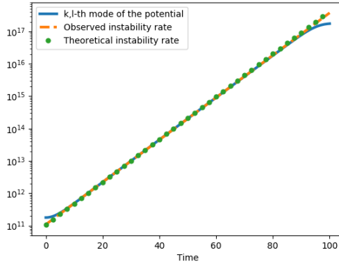
FIGURE 11. (Three-dimensional diocotron test-case) Instability rate observed compared to the theoretical one. Parameters: \lambda_p = 7 , \lambda_t = 600 , DG order p = 2 , \omega = 1.99 , n_p = 128 .
