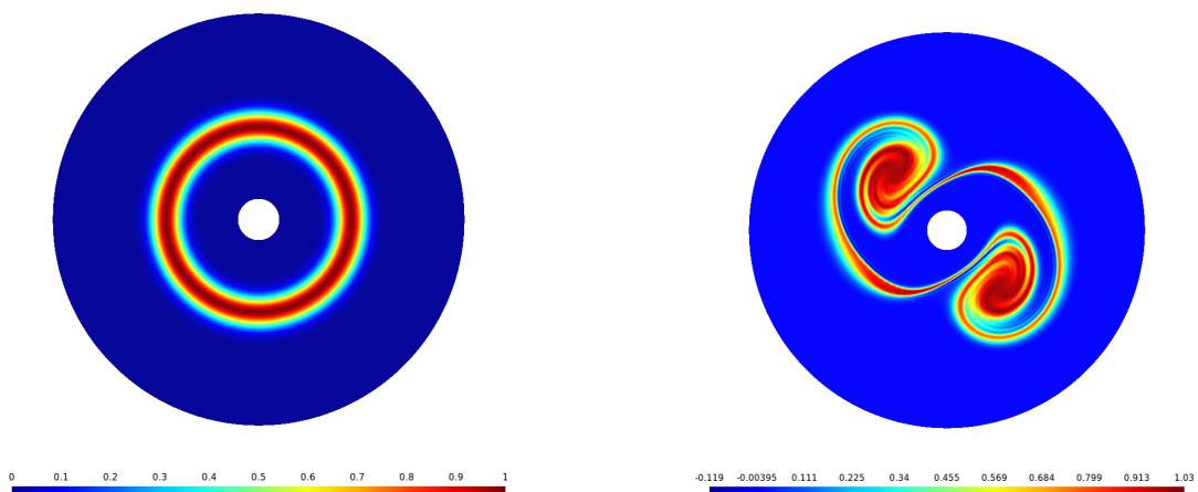
FIGURE 7. (Two-dimensional diocotron test-case) Density at t = 0 and t = 100 . Parameters: \lambda_p = 7 , DG order p = 2 , \Delta t = 0.0125 , \omega = 1.999 .
