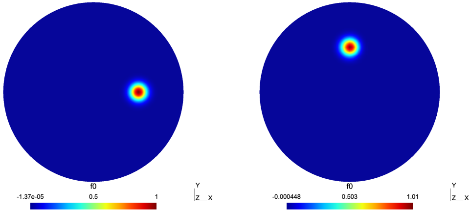
FIGURE 4. (Validation in two-dimension) Numerical solution at times t = 0 (left) and t = 2\pi (right) after the Gaussian pulse has done a quarter turn. Parameters of the kinetic solver: \Delta t = 2\pi/n_t with n_t = 1000 , \omega = 2 , \lambda_p = 1 and DG of order 2.
