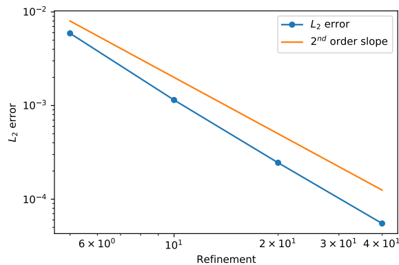
FIGURE 6. (Validation in three-dimension) L^2 error as a function of the refinement level. Parameters: \lambda_t = \lambda_p = 1 , DG order p = 2 .
