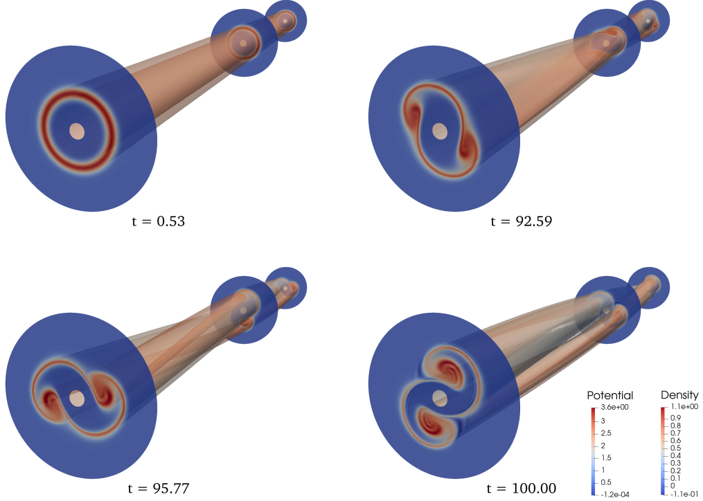
FIGURE 9. (Three-dimensional diocotron test-case) Four successive instants of the 3D solution showing cross sections of density colormaps and density isosurface colored by the potential. Parameters: \lambda_p = 7 , \lambda_t = 600 , DG order p = 2 , \omega = 1.99 , n_p = 65 .
