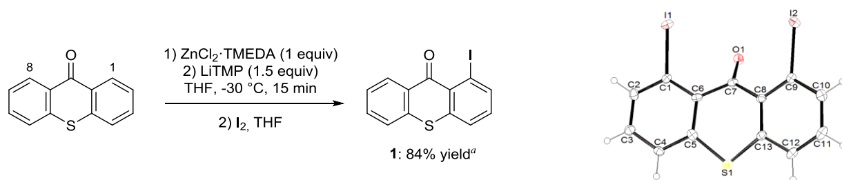
Scheme 1. Synthesis of 1-iodo-9-thioxanthone ( 1 ) and ORTEP diagram (50% probability) of the compound 1' . a 1,8-Diiido-9-thioxanthone ( 1' ) was also isolated in 10% yield.
