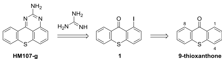
Figure 2. Retrosynthetic pathway of the PIM1 kinase inhibitor HM107-g [4].
