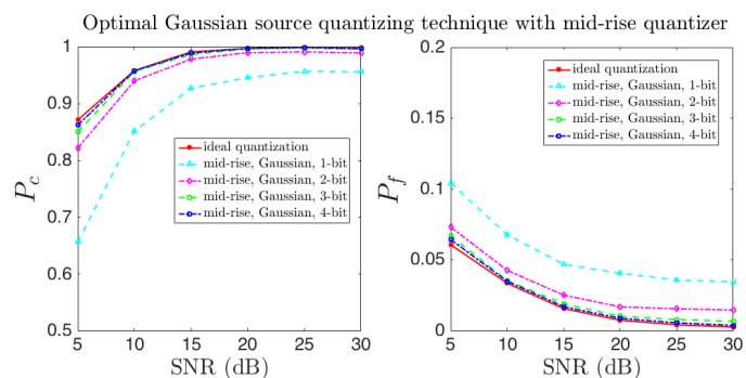
Fig. 3: Correct reconstruction and false alarm rates in function of SNRs (dB) obtained by the MWC with 1 to 4 bits common mid-rise quantizers applying optimal Gaussian source quantizing technique.
