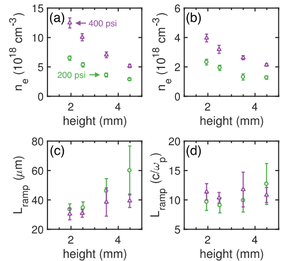
FIG. 3. Characteristics of the down ramp as a function of the plasma height. (a) Upper shelf density of the down ramp. (b) Lower shelf density of the down ramp. (c) Ramp length in real units. (d) Ramp length in normalized units. Each dot is an average, and the error bar represents the standard deviation of 20 shots. The purple triangles (green circles) are measured under a backing pressure of 400 (200) psi.
