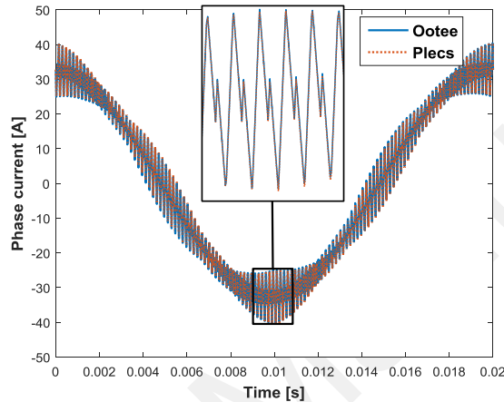
Fig. 4. Comparative of the output current for both simulation software.
