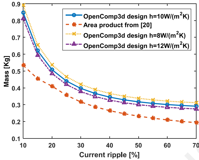
Fig. 12. Comparison of optimal results with classical product area versus current ripple.
