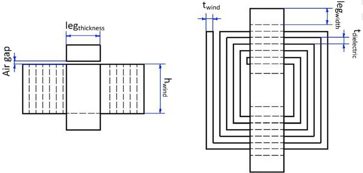
Fig. 7. Dimensions of the inductor.
