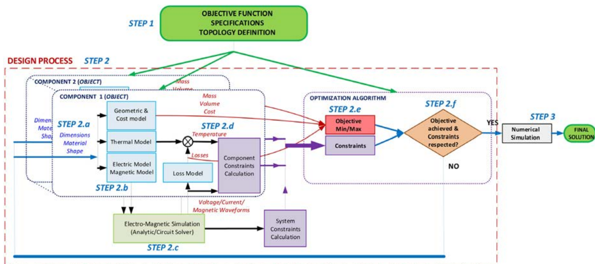
Fig. 5. Optimization algorithm process.
