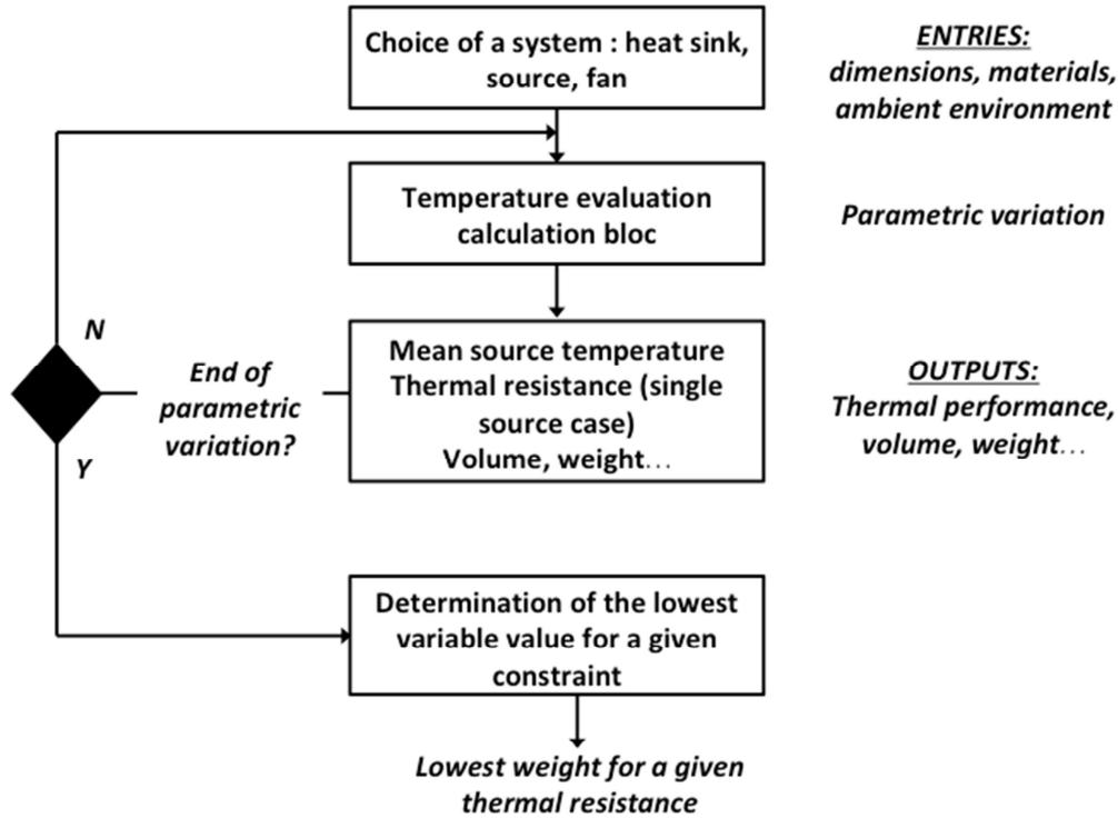
Fig. 9 : Optimization algorithm used to define the heat geometry with the lowest weight for a given thermal resistance value. The heat sink of Fig. 6 is used as a reference design for comparison, having a thermal resistance of 0.175K/W. Given the geometrical and mechanical constraints for the insertion of this heat sink in the real SiC converter, parameters were varied as presented in Table 1. The heat source is the same SiC module having 47mm width and 108mm length. The factor k , given by k = n_{FIN} \cdot T_{FIN} / W gives an idea of the fin thickness T_{FIN} .
