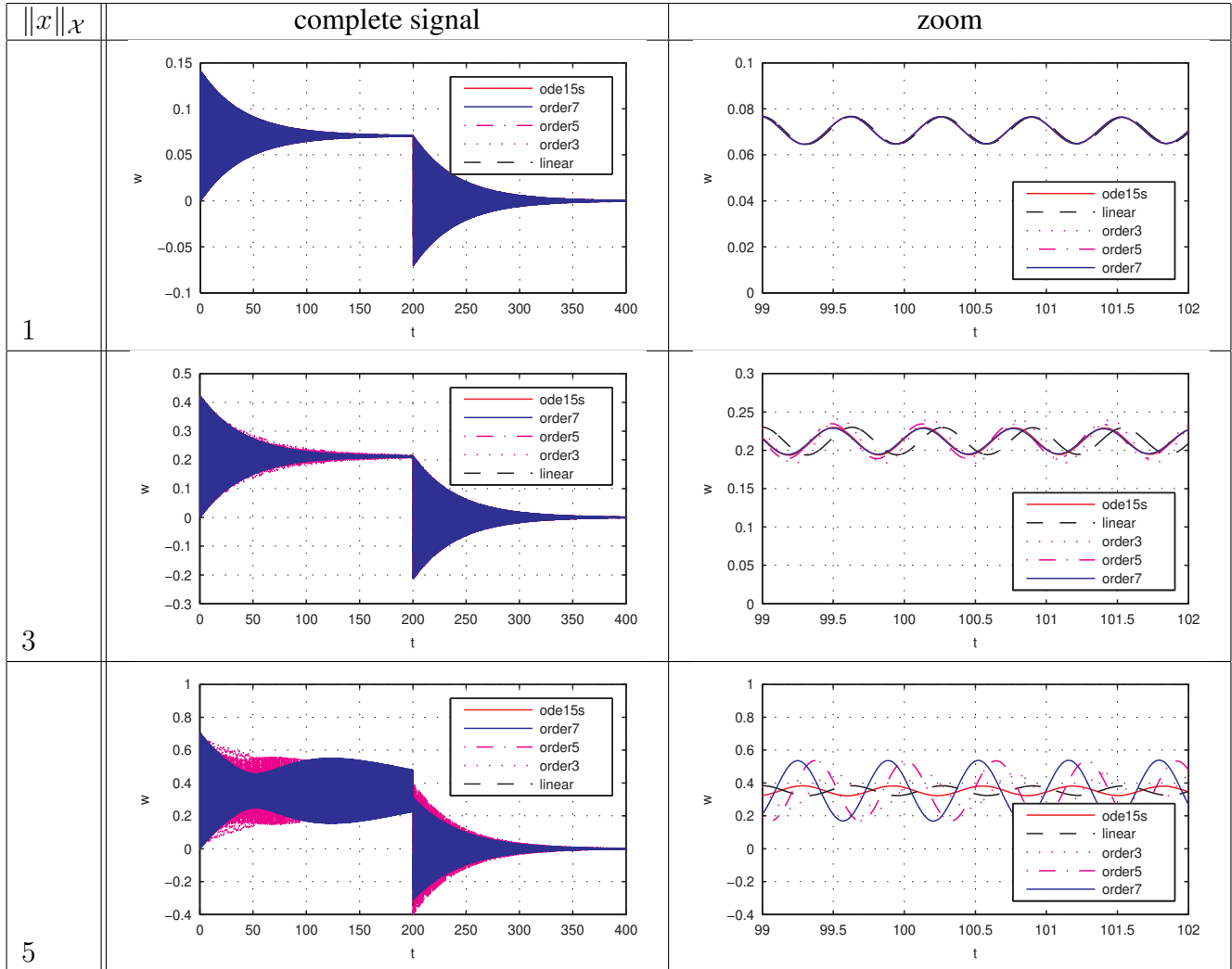
Figure 4: Simulations for configuration 2 (oscillating wooden beam)
