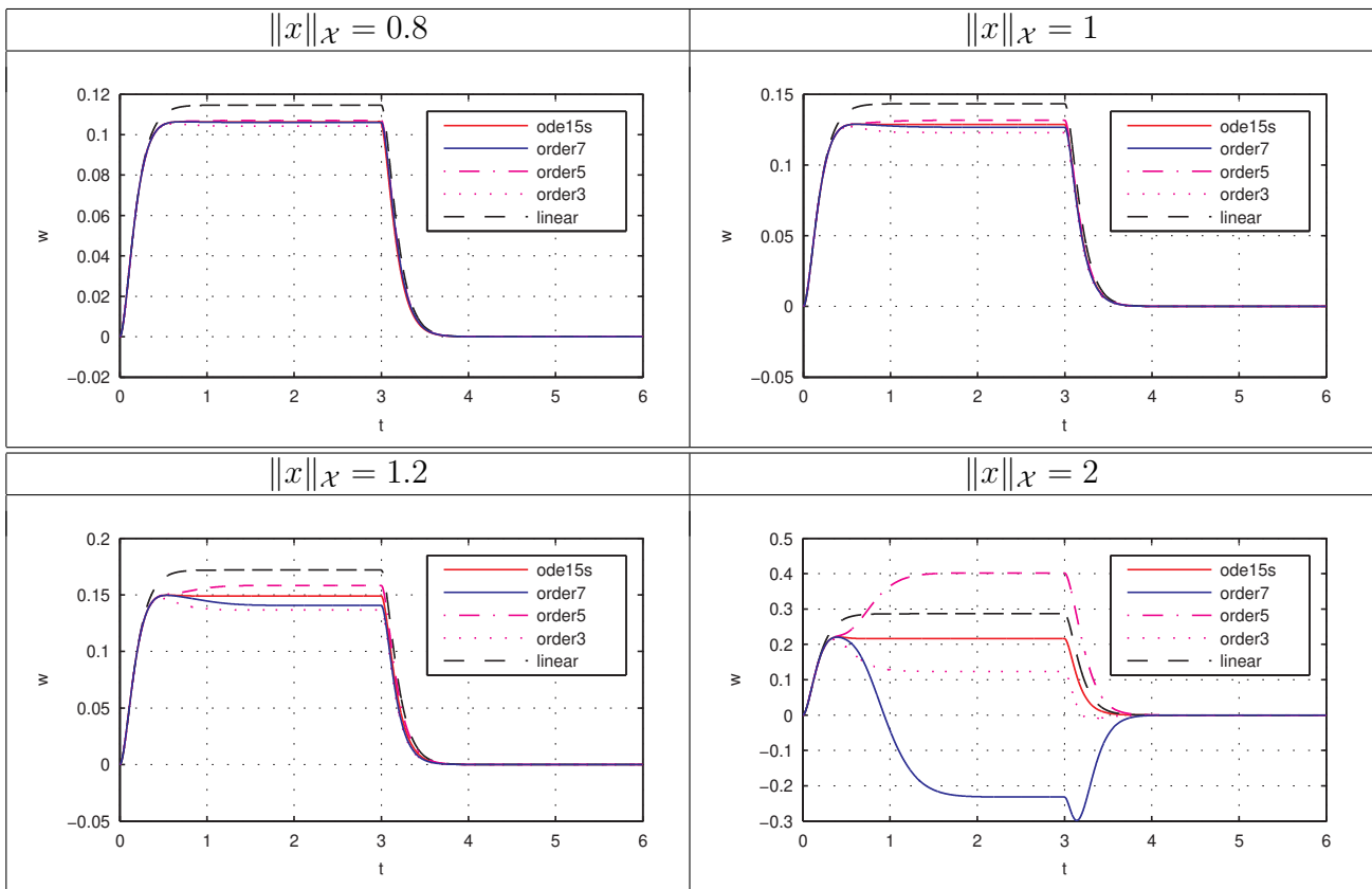
Figure 2: Simulations for configuration 1 (the reference is computed by the standard ODE solver ode15s, Matlab).
