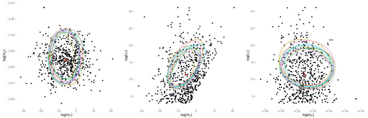
Fig. 6.3: Two-dimensional marginal distributions of the posterior distribution for section 6. In black, MCMC-ABC samples. The colored ellipses represent contours for EP-ABC approximate posteriors (scaled to span 4 times the standard deviation across the diameter). Each ellipse represents the results for a different run of EP-ABC. The posterior distribution exhibits extremely poor scaling (compare the range of \log m_1 to that of \log m_{21} ), and a truncated shape along some dimensions. Red triangles represent posterior mean computed from MCMC-ABC samples.
